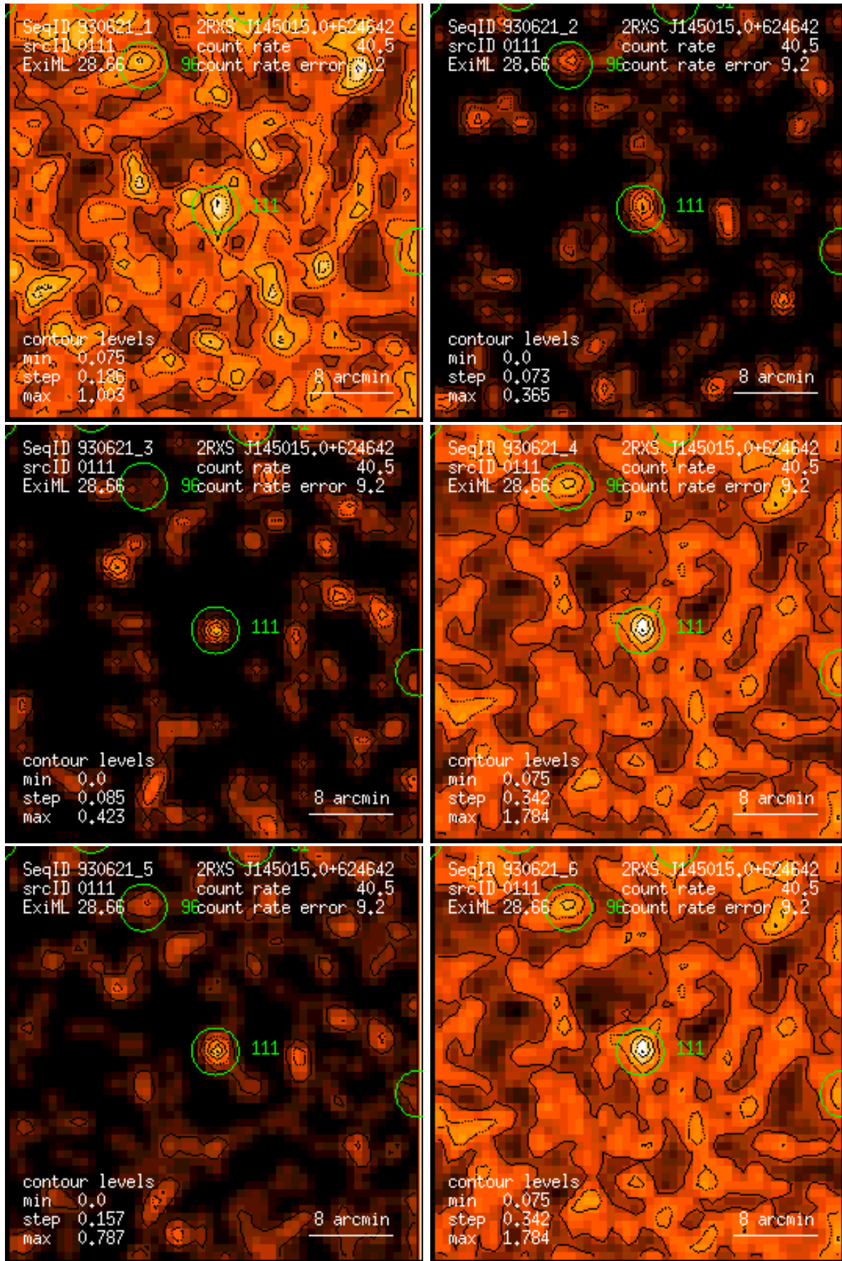
Figure 111: RASS 930621: detection 0111: band rate images, Gaussian filter: (1) PSPC channels 11 – 41, (2) 52 – 90, (3) 91 – 201, (4) 11 – 235, (5) 52 – 201, (6) 11 – 201. Broad band rates in counts/ks. Band rate contour levels in counts/ks/arcmin 2 .
