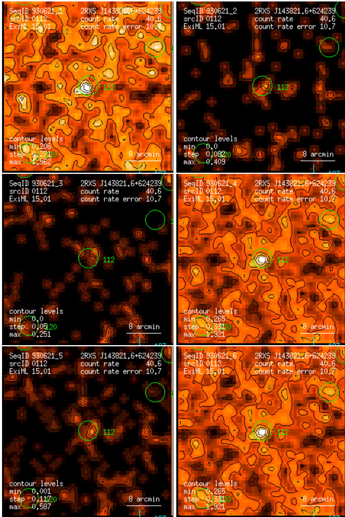
Figure 112: RASS 930621: detection 0112: band rate images, Gaussian filter: (1) PSPC channels 11 – 41, (2) 52 – 90, (3) 91 – 201, (4) 11 – 235, (5) 52 – 201, (6) 11 – 201. Broad band rates in counts/ks. Band rate contour levels in counts/ks/arcmin 2 .
