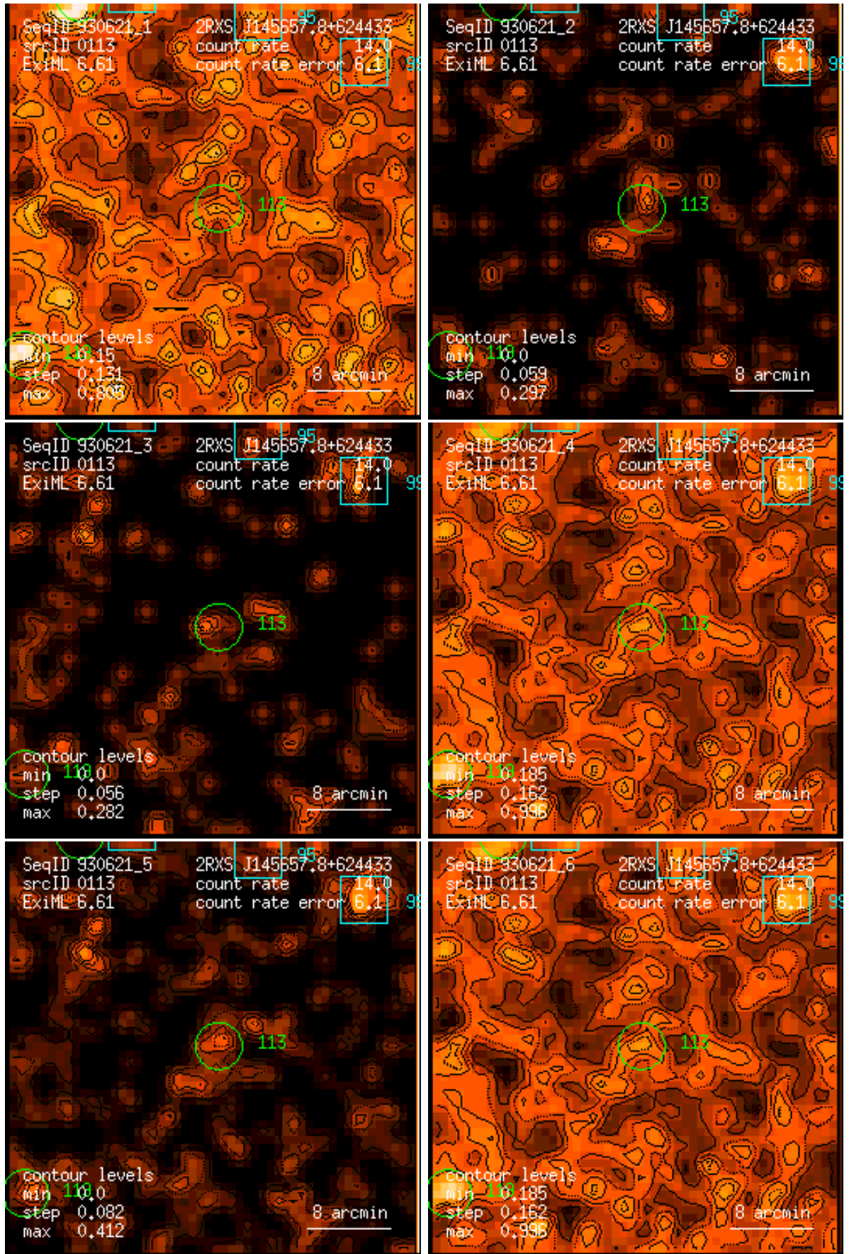
Figure 113: RASS 930621: detection 0113: band rate images, Gaussian filter: (1) PSPC channels 11 – 41, (2) 52 – 90, (3) 91 – 201, (4) 11 – 235, (5) 52 – 201, (6) 11 – 201. Broad band rates in counts/ks. Band rate contour levels in counts/ks/arcmin 2 .
