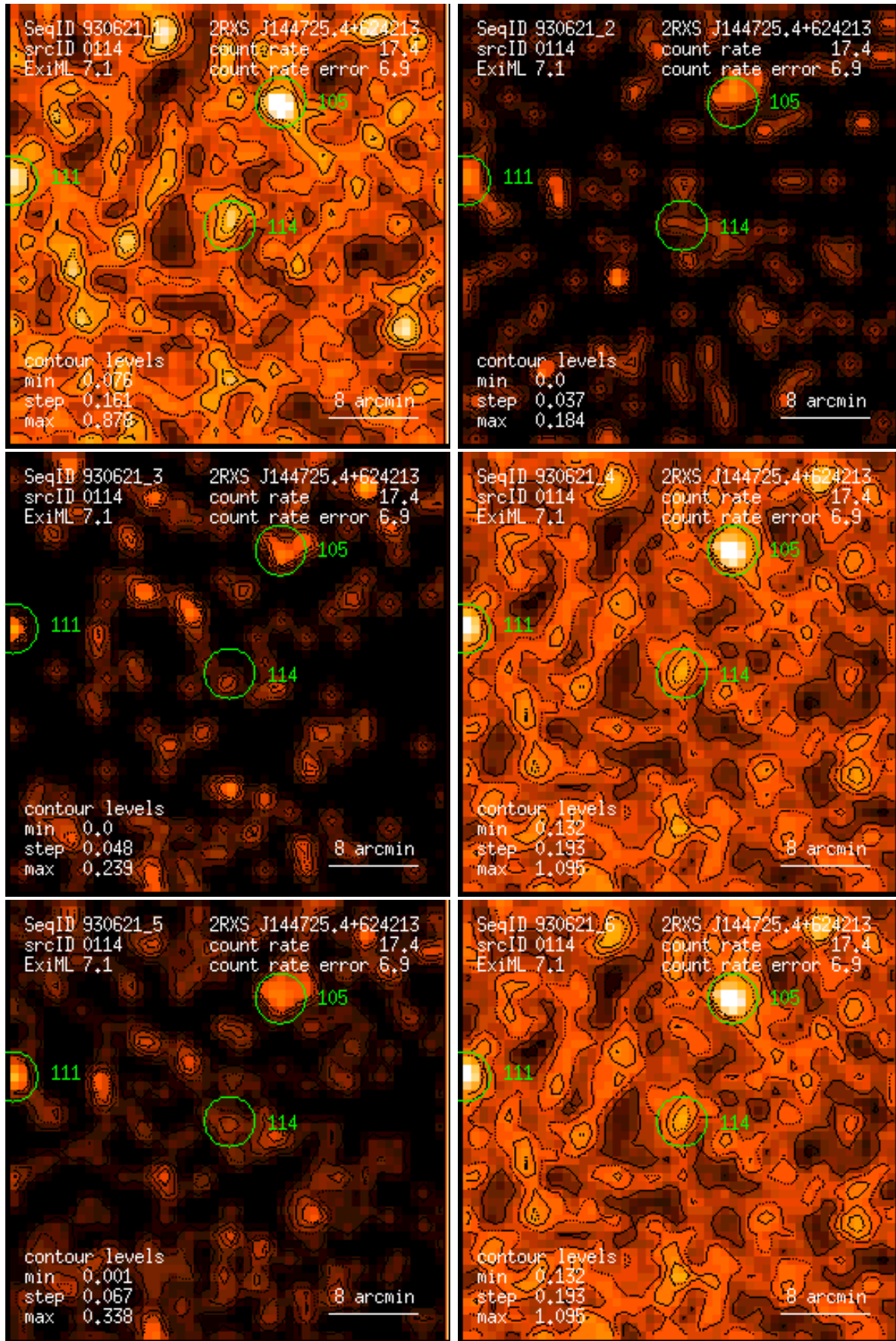
Figure 114: RASS 930621: detection 0114: band rate images, Gaussian filter: (1) PSPC channels 11 – 41, (2) 52 – 90, (3) 91 – 201, (4) 11 – 235, (5) 52 – 201, (6) 11 – 201. Broad band rates in counts/ks. Band rate contour levels in counts/ks/arcmin 2 .
