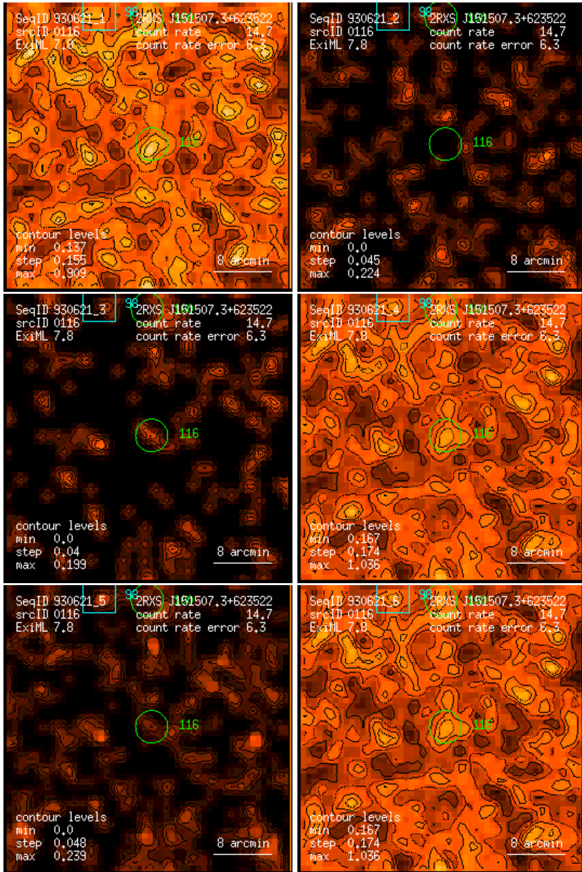
Figure 116: RASS 930621: detection 0116: band rate images, Gaussian filter: (1) PSPC channels 11 – 41, (2) 52 – 90, (3) 91 – 201, (4) 11 – 235, (5) 52 – 201, (6) 11 – 201. Broad band rates in counts/ks. Band rate contour levels in counts/ks/arcmin 2 .
