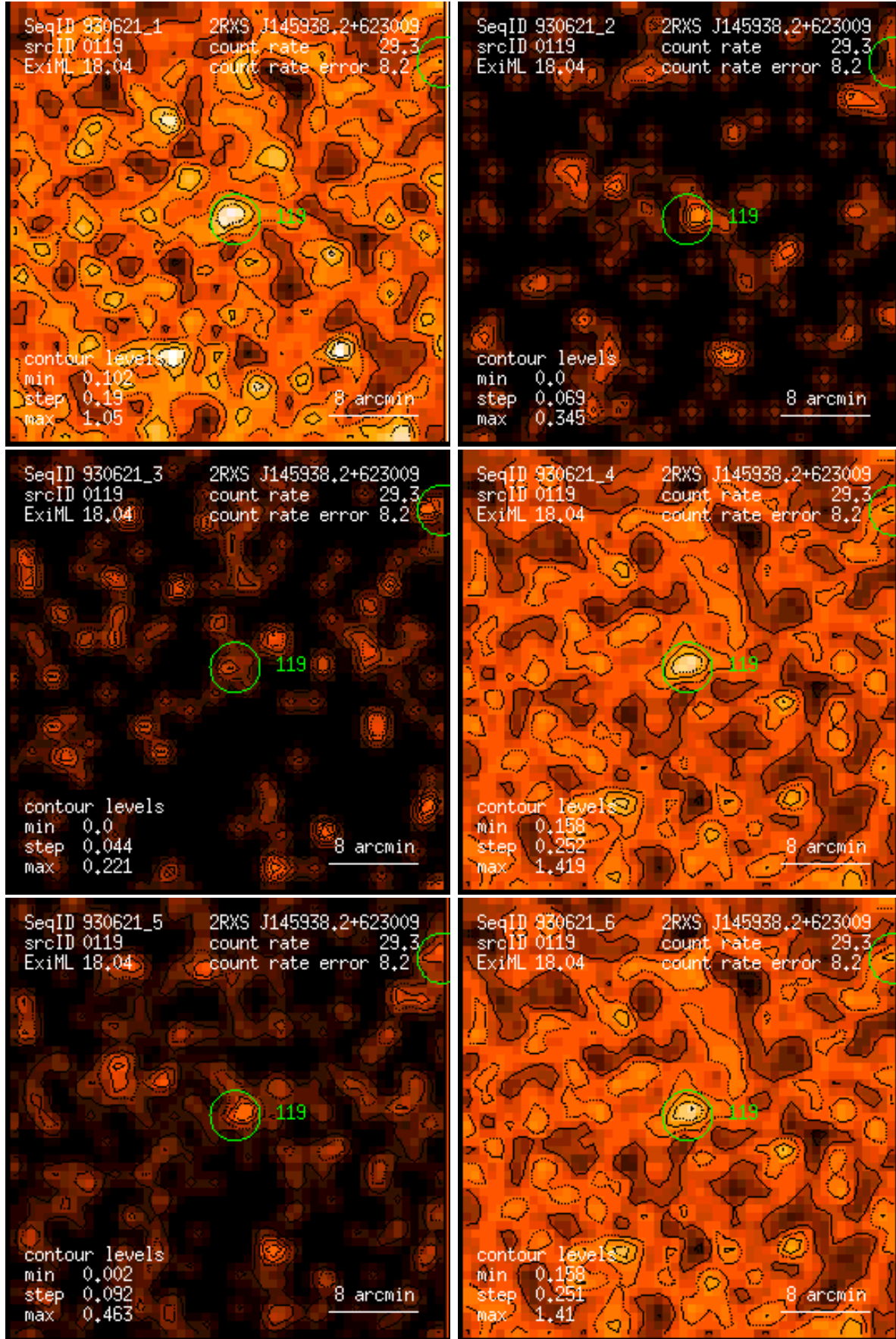
Figure 119: RASS 930621: detection 0119: band rate images, Gaussian filter: (1) PSPC channels 11 – 41, (2) 52 – 90, (3) 91 – 201, (4) 11 – 235, (5) 52 – 201, (6) 11 – 201. Broad band rates in counts/ks. Band rate contour levels in counts/ks/arcmin 2 .
