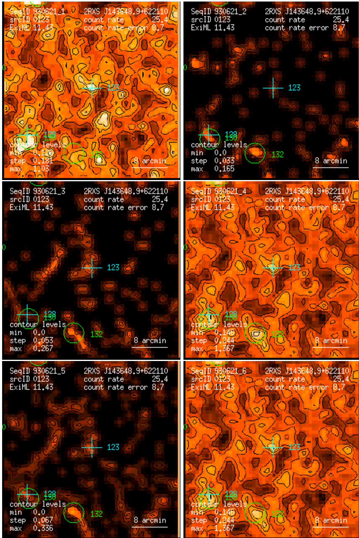
Figure 123: RASS 930621: detection 0123: band rate images, Gaussian filter: (1) PSPC channels 11 – 41, (2) 52 – 90, (3) 91 – 201, (4) 11 – 235, (5) 52 – 201, (6) 11 – 201. Broad band rates in counts/ks. Band rate contour levels in counts/ks/arcmin 2 .
