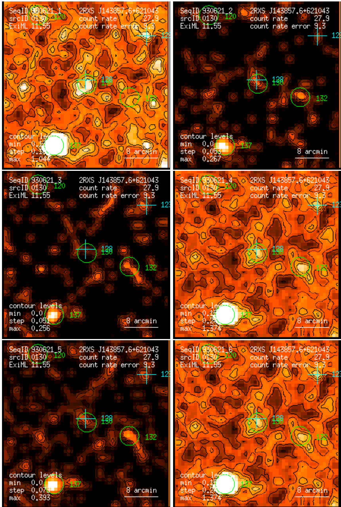
Figure 130: RASS 930621: detection 0130: band rate images, Gaussian filter: (1) PSPC channels 11 – 41, (2) 52 – 90, (3) 91 – 201, (4) 11 – 235, (5) 52 – 201, (6) 11 – 201. Broad band rates in counts/ks. Band rate contour levels in counts/ks/arcmin 2 .
