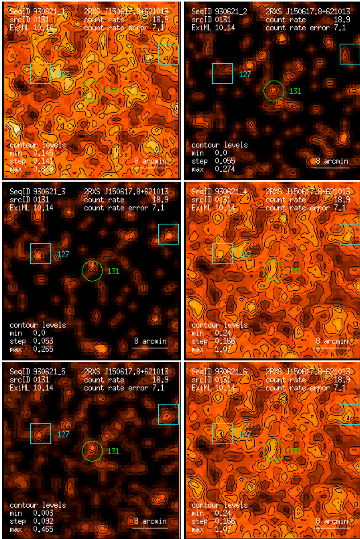
Figure 131: RASS 930621: detection 0131: band rate images, Gaussian filter: (1) PSPC channels 11 – 41, (2) 52 – 90, (3) 91 – 201, (4) 11 – 235, (5) 52 – 201, (6) 11 – 201. Broad band rates in counts/ks. Band rate contour levels in counts/ks/arcmin 2 .
