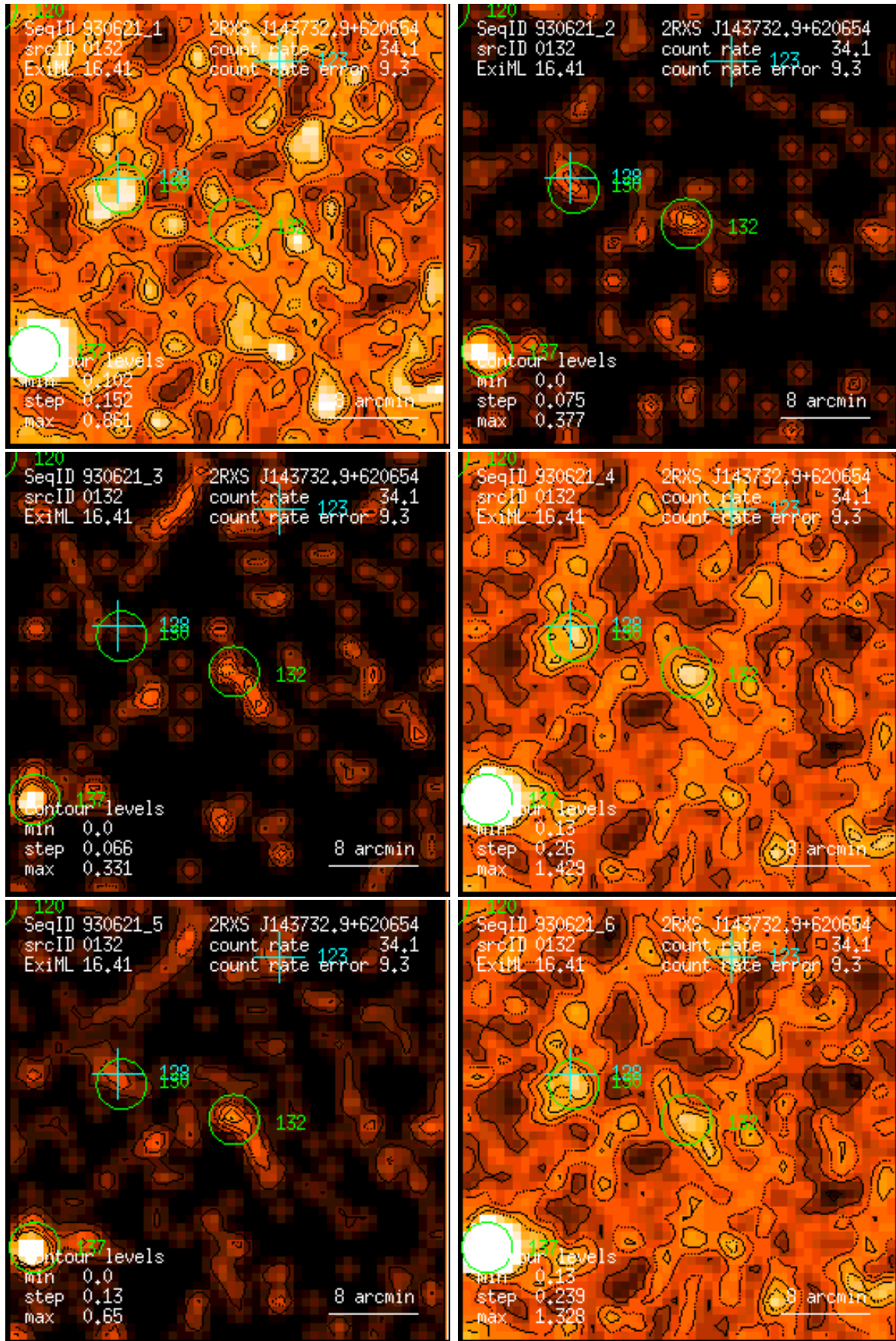
Figure 132: RASS 930621: detection 0132: band rate images, Gaussian filter: (1) PSPC channels 11 – 41, (2) 52 – 90, (3) 91 – 201, (4) 11 – 235, (5) 52 – 201, (6) 11 – 201. Broad band rates in counts/ks. Band rate contour levels in counts/ks/arcmin 2 .
