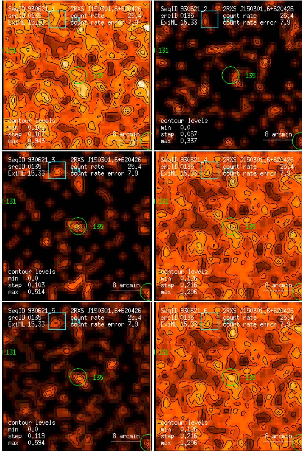
Figure 135: RASS 930621: detection 0135: band rate images, Gaussian filter: (1) PSPC channels 11 – 41, (2) 52 – 90, (3) 91 – 201, (4) 11 – 235, (5) 52 – 201, (6) 11 – 201. Broad band rates in counts/ks. Band rate contour levels in counts/ks/arcmin 2 .
