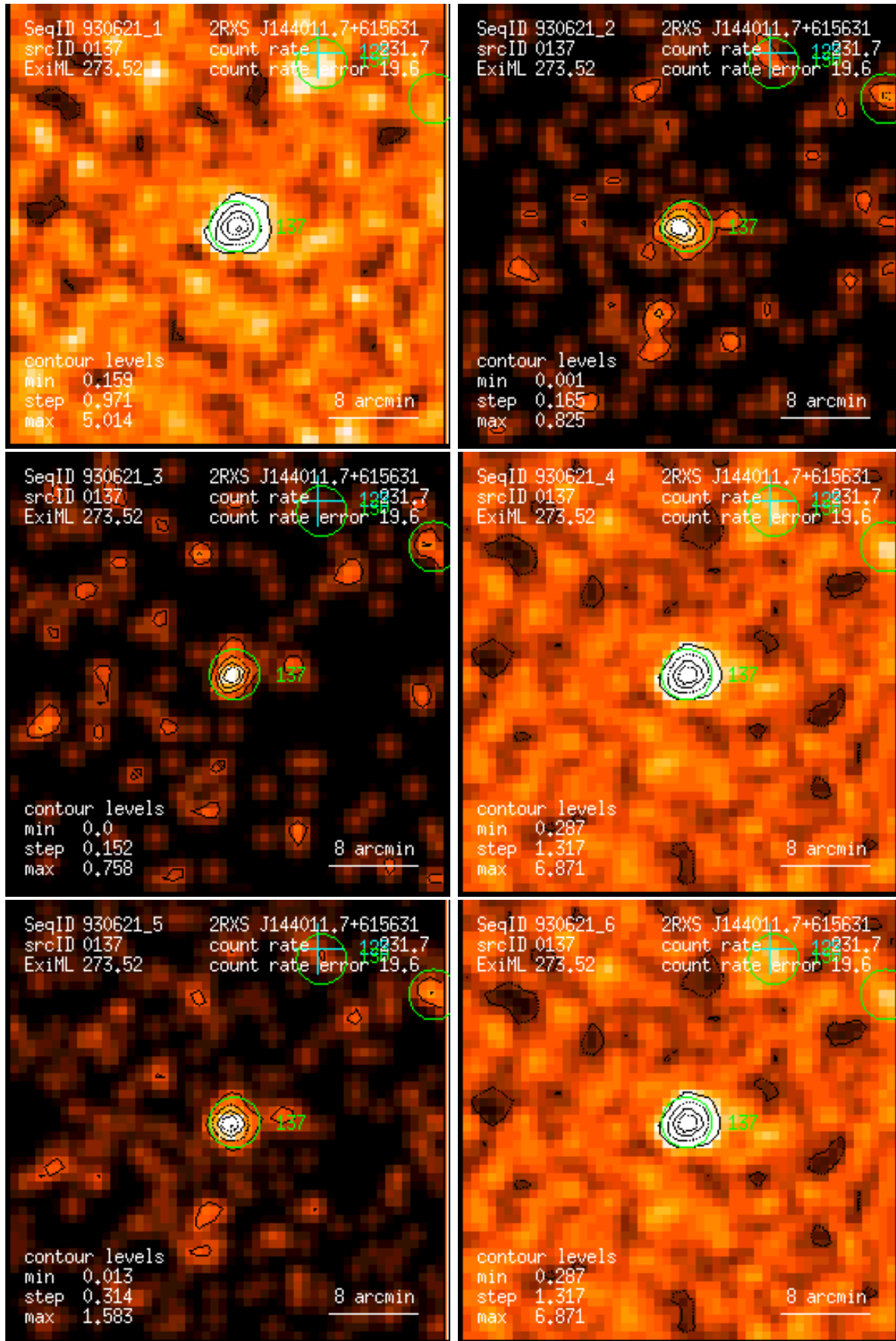
Figure 137: RASS 930621: detection 0137: band rate images, Gaussian filter: (1) PSPC channels 11 – 41, (2) 52 – 90, (3) 91 – 201, (4) 11 – 235, (5) 52 – 201, (6) 11 – 201. Broad band rates in counts/ks. Band rate contour levels in counts/ks/arcmin 2 .
