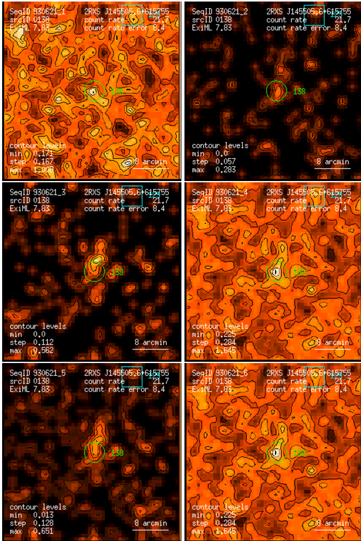
Figure 138: RASS 930621: detection 0138: band rate images, Gaussian filter: (1) PSPC channels 11 – 41, (2) 52 – 90, (3) 91 – 201, (4) 11 – 235, (5) 52 – 201, (6) 11 – 201. Broad band rates in counts/ks. Band rate contour levels in counts/ks/arcmin 2 .
