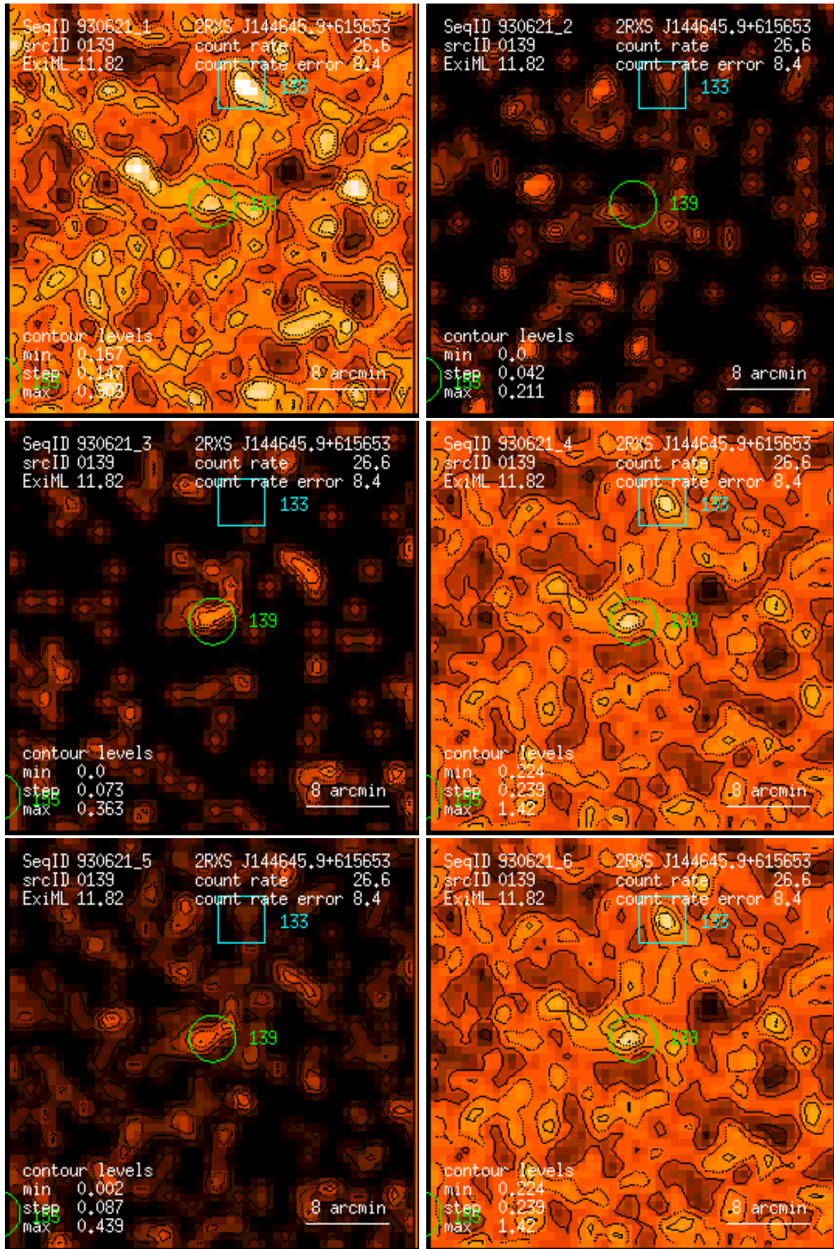
Figure 139: RASS 930621: detection 0139: band rate images, Gaussian filter: (1) PSPC channels 11 – 41, (2) 52 – 90, (3) 91 – 201, (4) 11 – 235, (5) 52 – 201, (6) 11 – 201. Broad band rates in counts/ks. Band rate contour levels in counts/ks/arcmin 2 .
