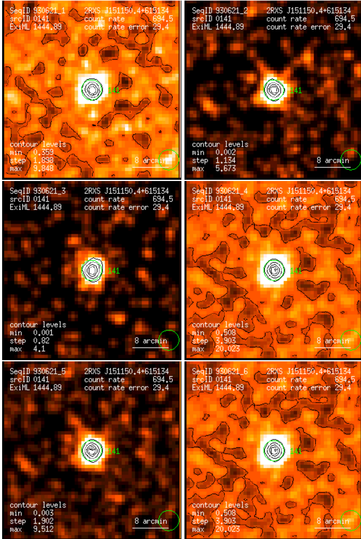
Figure 141: RASS 930621: detection 0141: band rate images, Gaussian filter: (1) PSPC channels 11 – 41, (2) 52 – 90, (3) 91 – 201, (4) 11 – 235, (5) 52 – 201, (6) 11 – 201. Broad band rates in counts/ks. Band rate contour levels in counts/ks/arcmin 2 .
