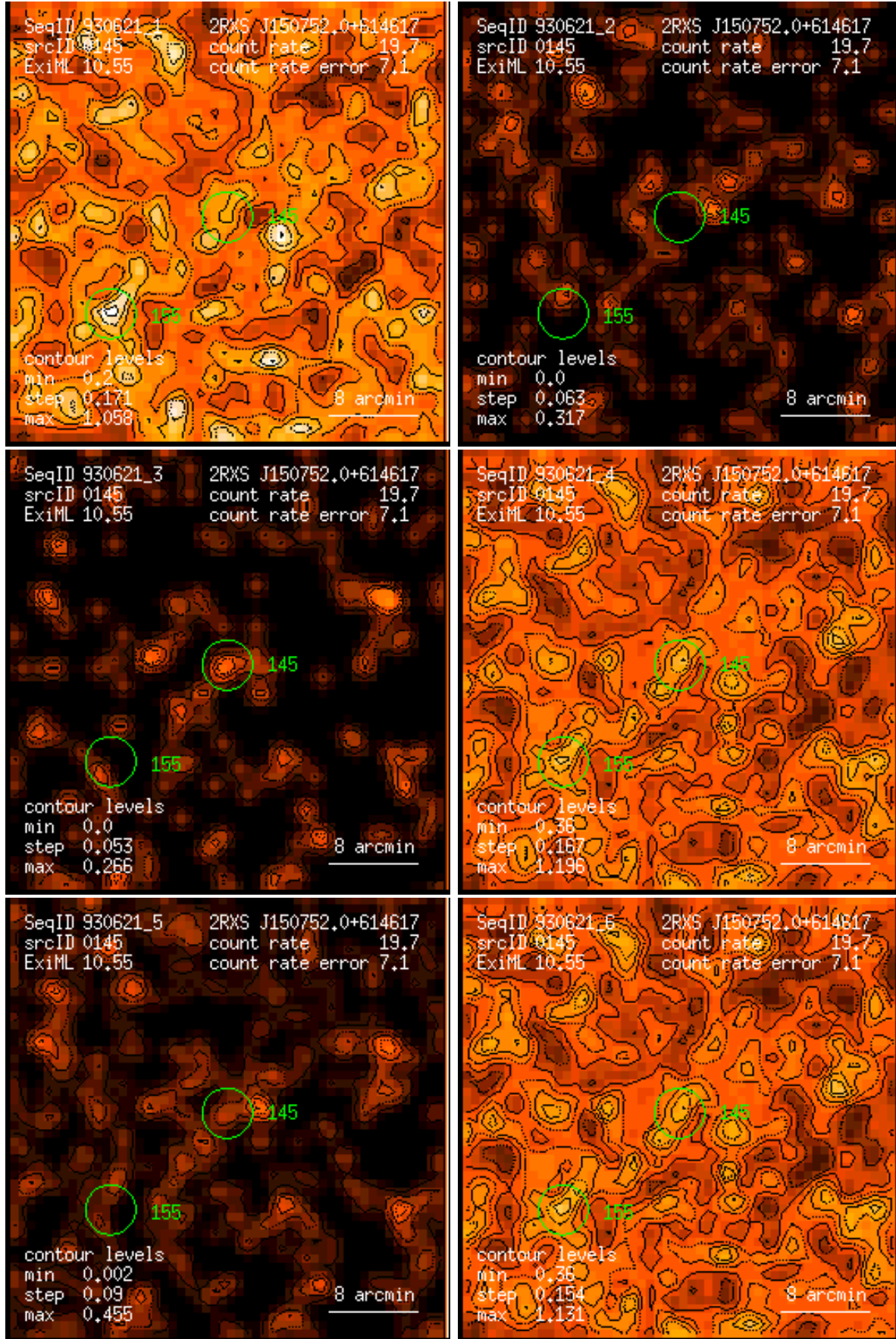
Figure 145: RASS 930621: detection 0145: band rate images, Gaussian filter: (1) PSPC channels 11 – 41, (2) 52 – 90, (3) 91 – 201, (4) 11 – 235, (5) 52 – 201, (6) 11 – 201. Broad band rates in counts/ks. Band rate contour levels in counts/ks/arcmin 2 .
