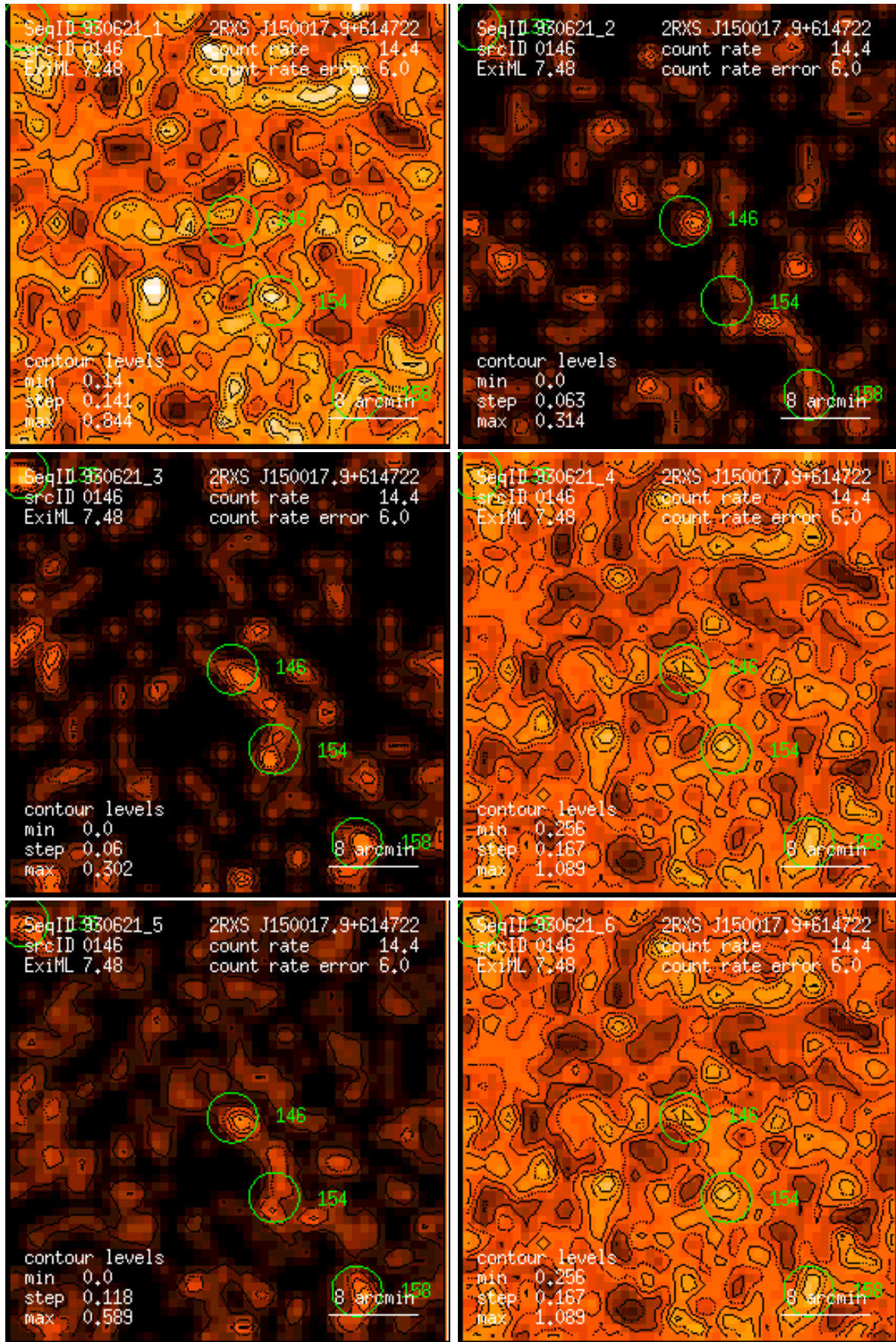
Figure 146: RASS 930621: detection 0146: band rate images, Gaussian filter: (1) PSPC channels 11 – 41, (2) 52 – 90, (3) 91 – 201, (4) 11 – 235, (5) 52 – 201, (6) 11 – 201. Broad band rates in counts/ks. Band rate contour levels in counts/ks/arcmin 2 .
