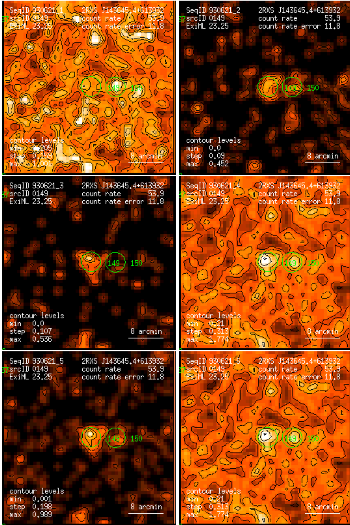
Figure 149: RASS 930621: detection 0149: band rate images, Gaussian filter: (1) PSPC channels 11 – 41, (2) 52 – 90, (3) 91 – 201, (4) 11 – 235, (5) 52 – 201, (6) 11 – 201. Broad band rates in counts/ks. Band rate contour levels in counts/ks/arcmin 2 .
