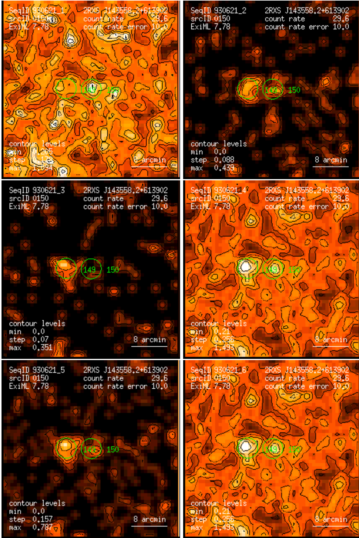
Figure 150: RASS 930621: detection 0150: band rate images, Gaussian filter: (1) PSPC channels 11 – 41, (2) 52 – 90, (3) 91 – 201, (4) 11 – 235, (5) 52 – 201, (6) 11 – 201. Broad band rates in counts/ks. Band rate contour levels in counts/ks/arcmin 2 .
