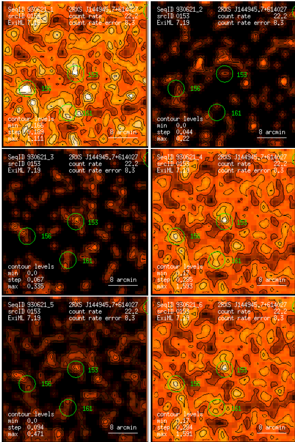
Figure 153: RASS 930621: detection 0153: band rate images, Gaussian filter: (1) PSPC channels 11 – 41, (2) 52 – 90, (3) 91 – 201, (4) 11 – 235, (5) 52 – 201, (6) 11 – 201. Broad band rates in counts/ks. Band rate contour levels in counts/ks/arcmin 2 .
