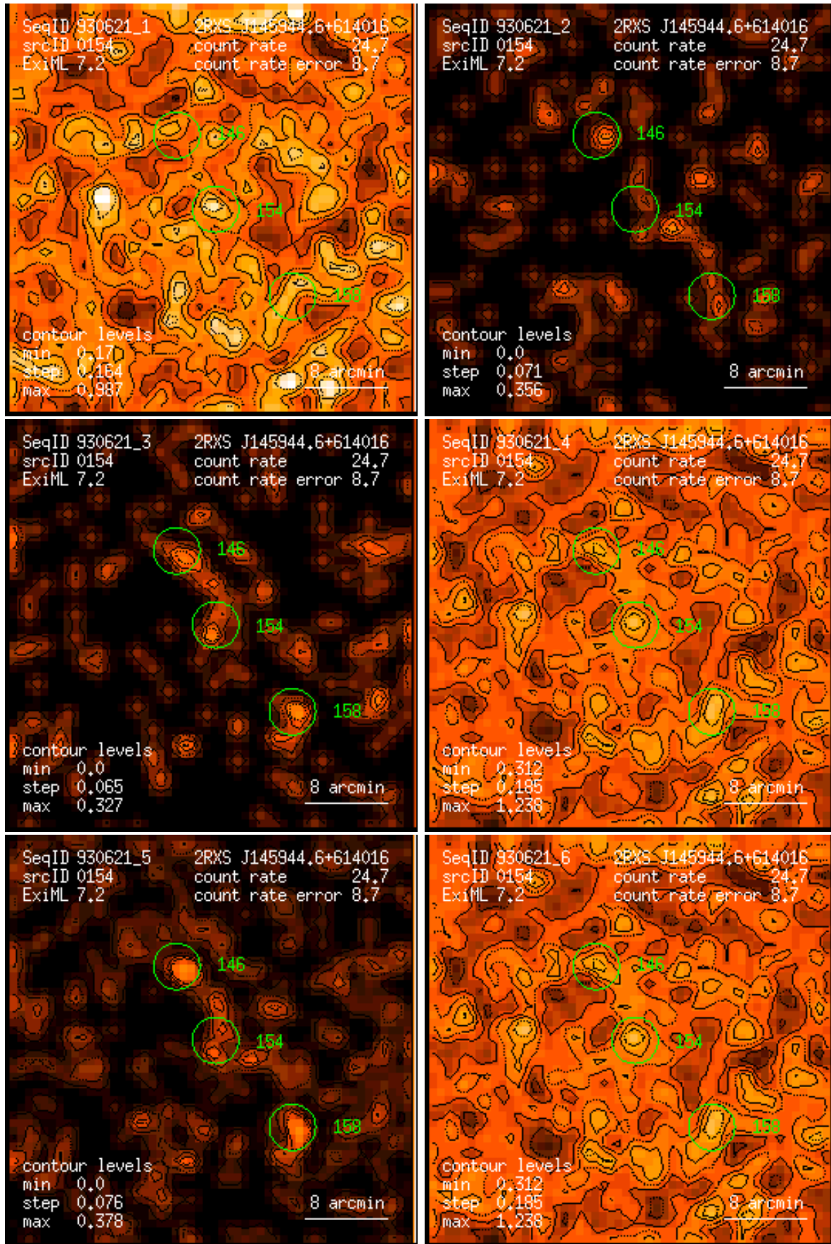
Figure 154: RASS 930621: detection 0154: band rate images, Gaussian filter: (1) PSPC channels 11 – 41, (2) 52 – 90, (3) 91 – 201, (4) 11 – 235, (5) 52 – 201, (6) 11 – 201. Broad band rates in counts/ks. Band rate contour levels in counts/ks/arcmin 2 .
