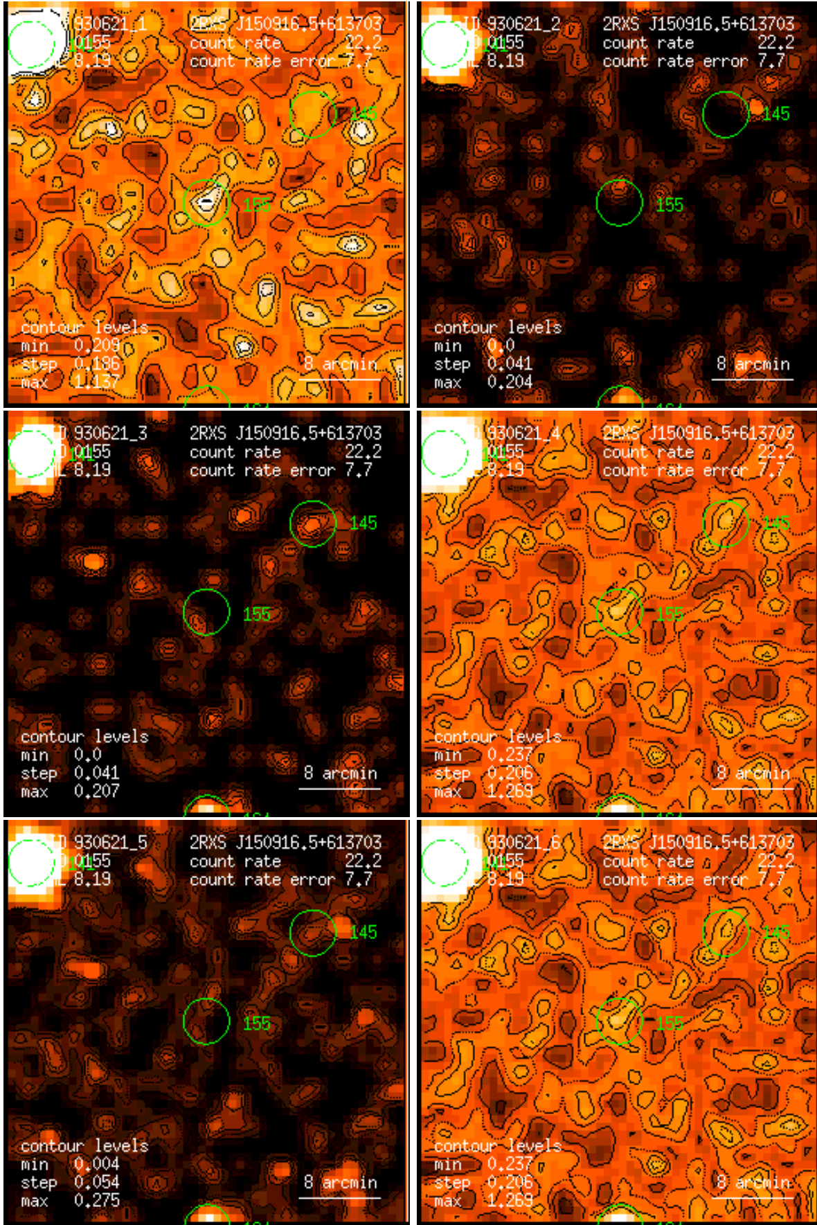
Figure 155: RASS 930621: detection 0155: band rate images, Gaussian filter: (1) PSPC channels 11 – 41, (2) 52 – 90, (3) 91 – 201, (4) 11 – 235, (5) 52 – 201, (6) 11 – 201. Broad band rates in counts/ks. Band rate contour levels in counts/ks/arcmin 2 .
