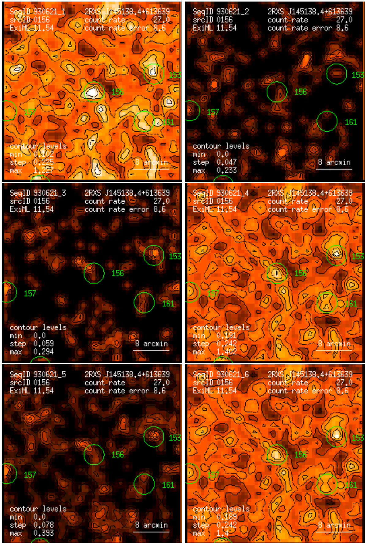
Figure 156: RASS 930621: detection 0156: band rate images, Gaussian filter: (1) PSPPC channels 11 – 41, (2) 52 – 90, (3) 91 – 201, (4) 11 – 235, (5) 52 – 201, (6) 11 – 201. Broad band rates in counts/ks. Band rate contour levels in counts/ks/arcmin 2 .
