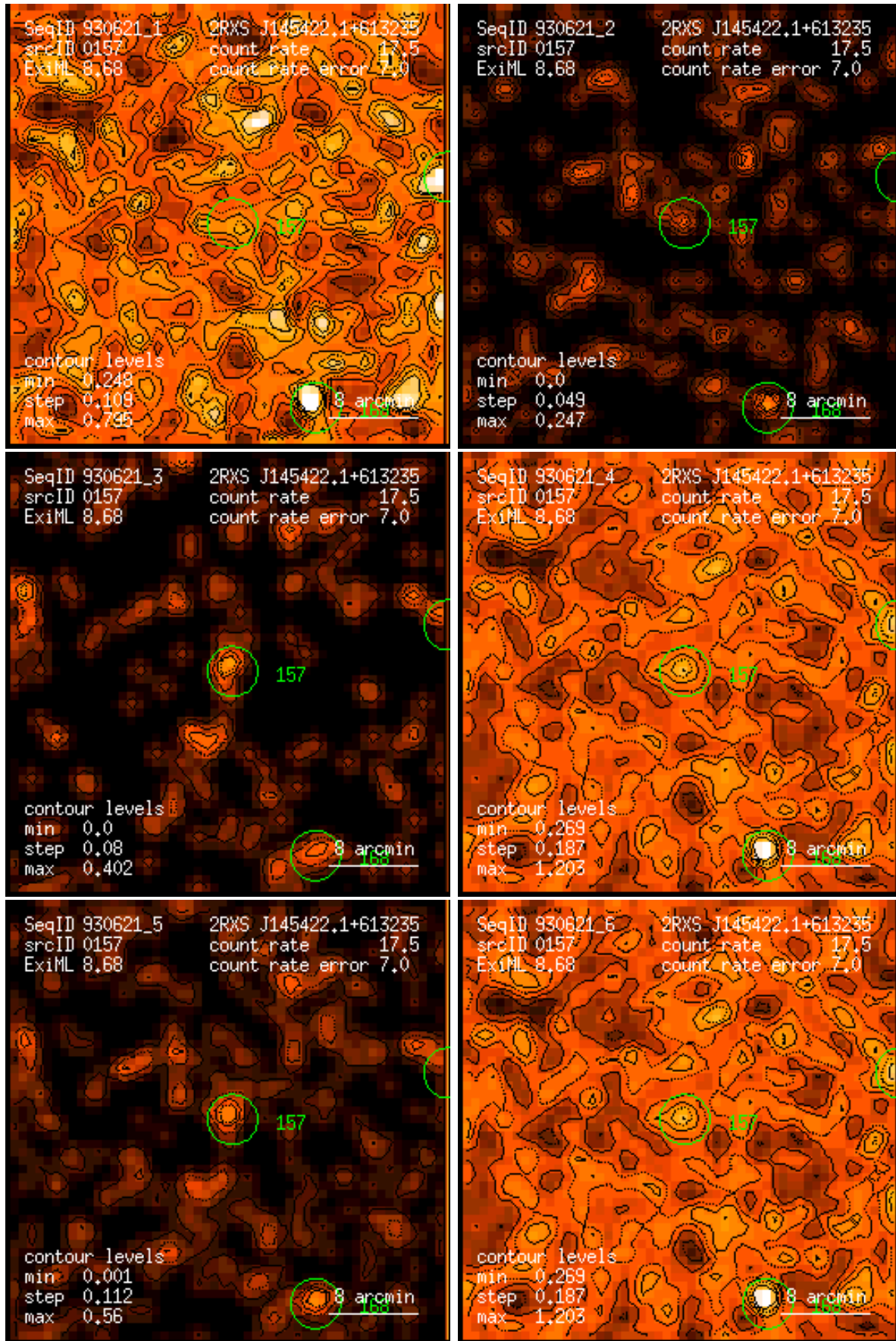
Figure 157: RASS 930621: detection 0157: band rate images, Gaussian filter: (1) PSPC channels 11 – 41, (2) 52 – 90, (3) 91 – 201, (4) 11 – 235, (5) 52 – 201, (6) 11 – 201. Broad band rates in counts/ks. Band rate contour levels in counts/ks/arcmin 2 .
