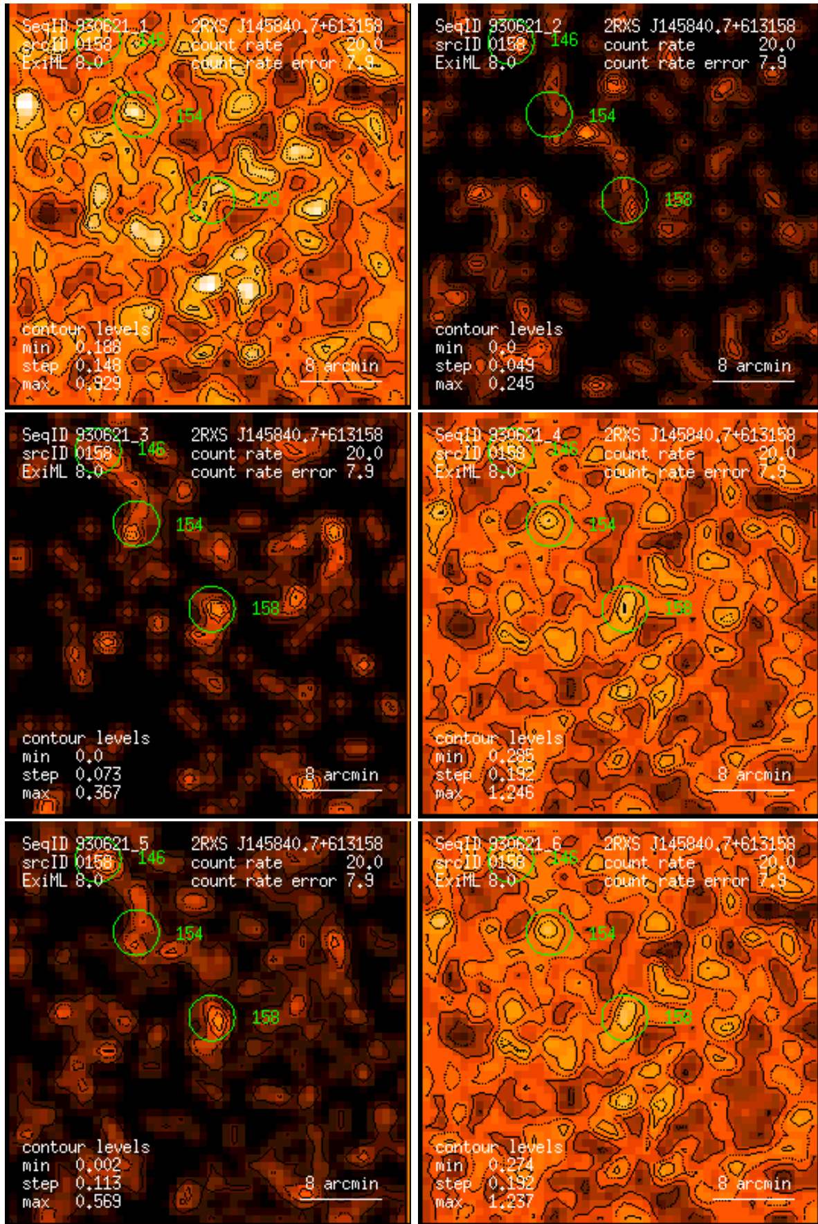
Figure 158: RASS 930621: detection 0158: band rate images, Gaussian filter: (1) PSPC channels 11 – 41, (2) 52 – 90, (3) 91 – 201, (4) 11 – 235, (5) 52 – 201, (6) 11 – 201. Broad band rates in counts/ks. Band rate contour levels in counts/ks/arcmin 2 .
