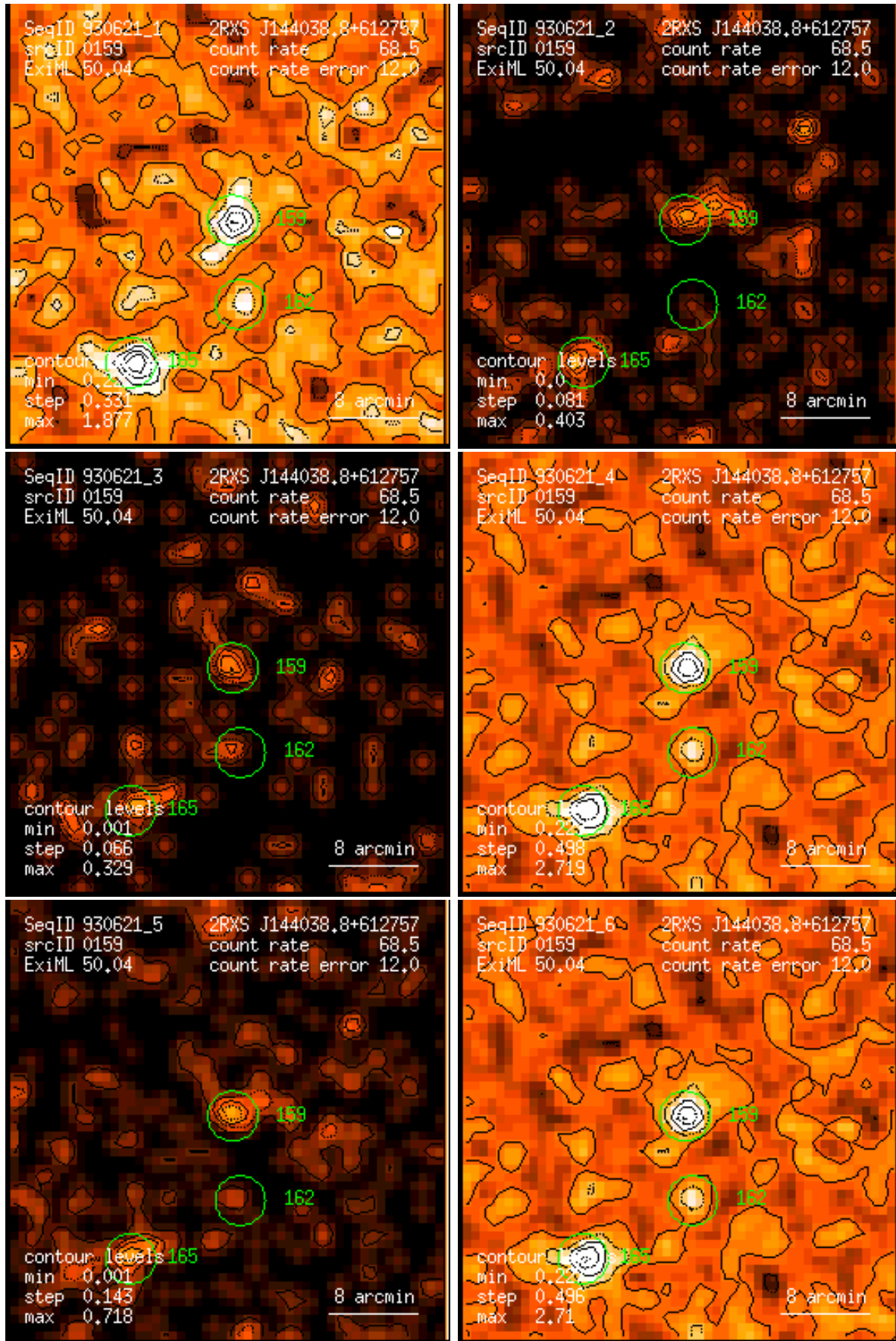
Figure 159: RASS 930621: detection 0159: band rate images, Gaussian filter: (1) PSPC channels 11 – 41, (2) 52 – 90, (3) 91 – 201, (4) 11 – 235, (5) 52 – 201, (6) 11 – 201. Broad band rates in counts/ks. Band rate contour levels in counts/ks/arcmin 2 .
