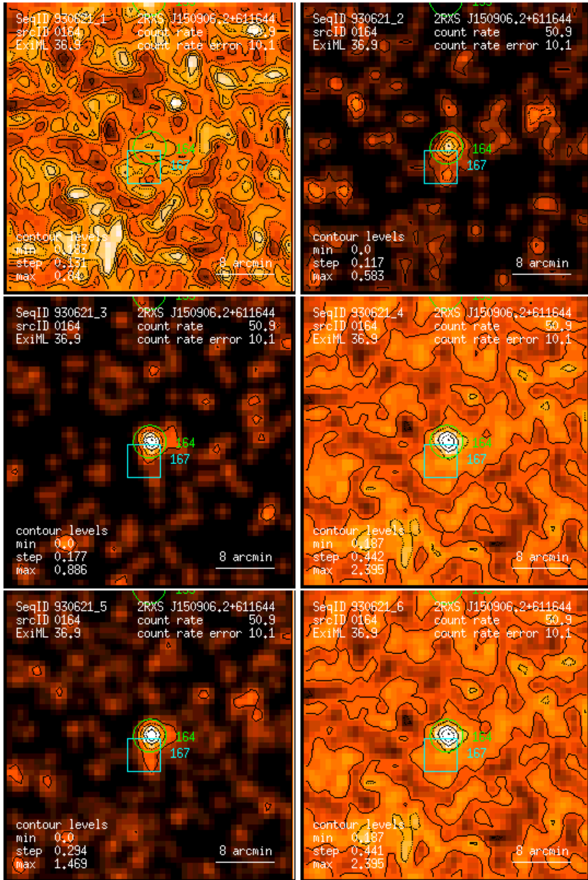
Figure 164: RASS 930621: detection 0164: band rate images, Gaussian filter: (1) PSPC channels 11 – 41, (2) 52 – 90, (3) 91 – 201, (4) 11 – 235, (5) 52 – 201, (6) 11 – 201. Broad band rates in counts/ks. Band rate contour levels in counts/ks/arcmin 2 .
