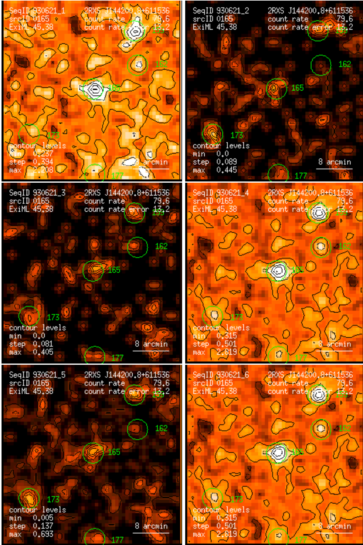
Figure 165: RASS 930621: detection 0165: band rate images, Gaussian filter: (1) PSPC channels 11 – 41, (2) 52 – 90, (3) 91 – 201, (4) 11 – 235, (5) 52 – 201, (6) 11 – 201. Broad band rates in counts/ks. Band rate contour levels in counts/ks/arcmin 2 .
