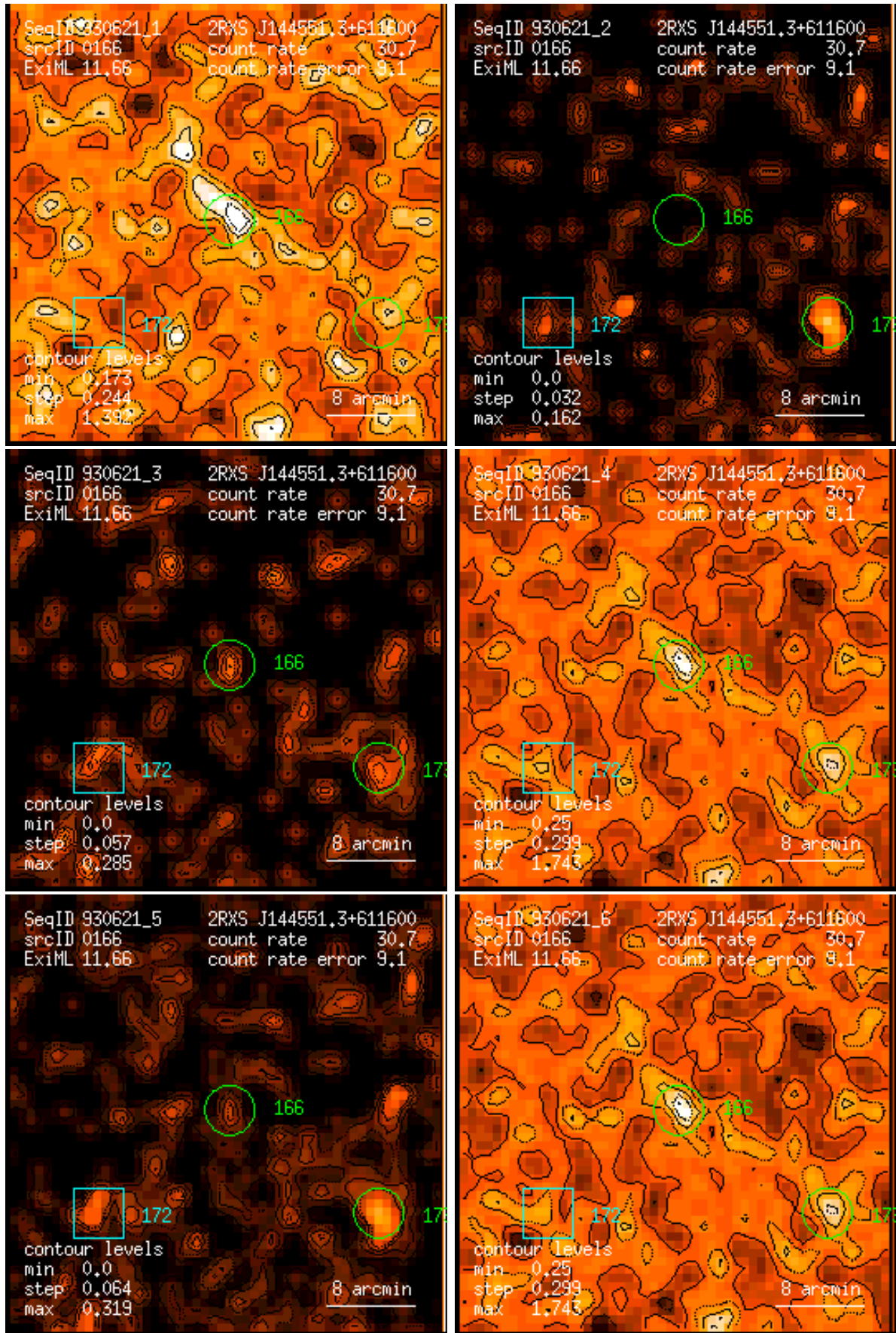
Figure 166: RASS 930621: detection 0166: band rate images, Gaussian filter: (1) PSPC channels 11 – 41, (2) 52 – 90, (3) 91 – 201, (4) 11 – 235, (5) 52 – 201, (6) 11 – 201. Broad band rates in counts/ks. Band rate contour levels in counts/ks/arcmin 2 .
