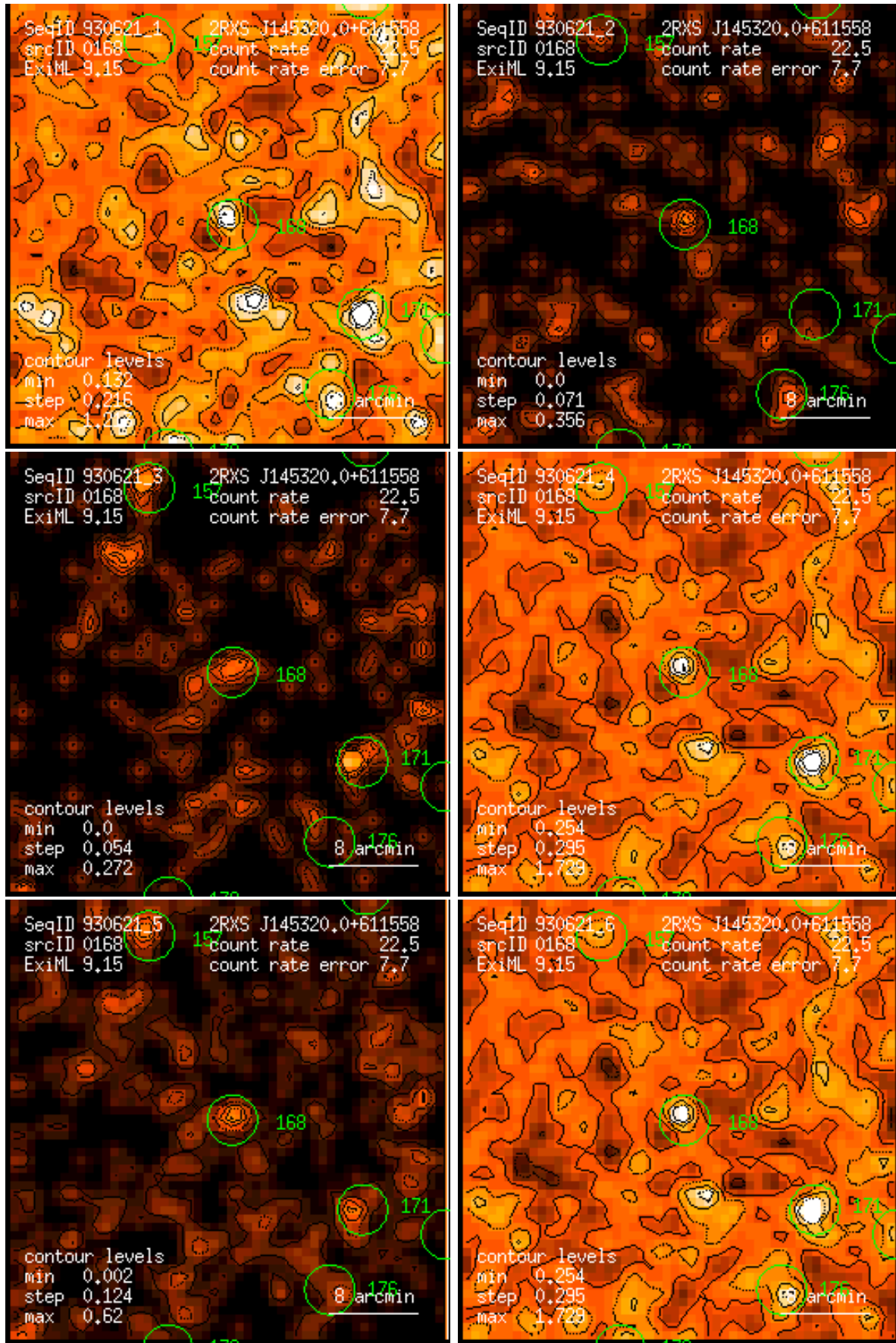
Figure 168: RASS 930621: detection 0168: band rate images, Gaussian filter: (1) PSPC channels 11 – 41, (2) 52 – 90, (3) 91 – 201, (4) 11 – 235, (5) 52 – 201, (6) 11 – 201. Broad band rates in counts/ks. Band rate contour levels in counts/ks/arcmin 2 .
