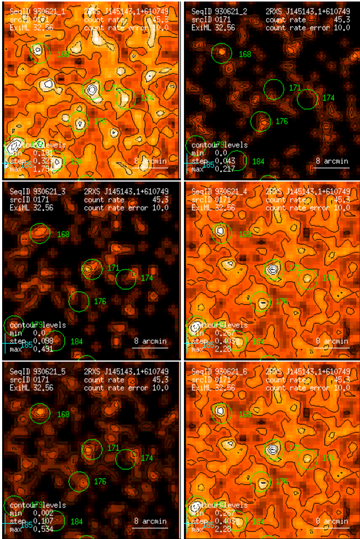
Figure 171: RASS 930621: detection 0171: band rate images, Gaussian filter: (1) PSPC channels 11 – 41, (2) 52 – 90, (3) 91 – 201, (4) 11 – 235, (5) 52 – 201, (6) 11 – 201. Broad band rates in counts/ks. Band rate contour levels in counts/ks/arcmin 2 .
