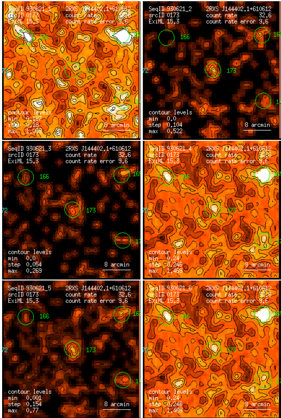
Figure 173: RASS 930621: detection 0173: band rate images, Gaussian filter: (1) PSPC channels 11 – 41, (2) 52 – 90, (3) 91 – 201, (4) 11 – 235, (5) 52 – 201, (6) 11 – 201. Broad band rates in counts/ks. Band rate contour levels in counts/ks/arcmin 2 .
