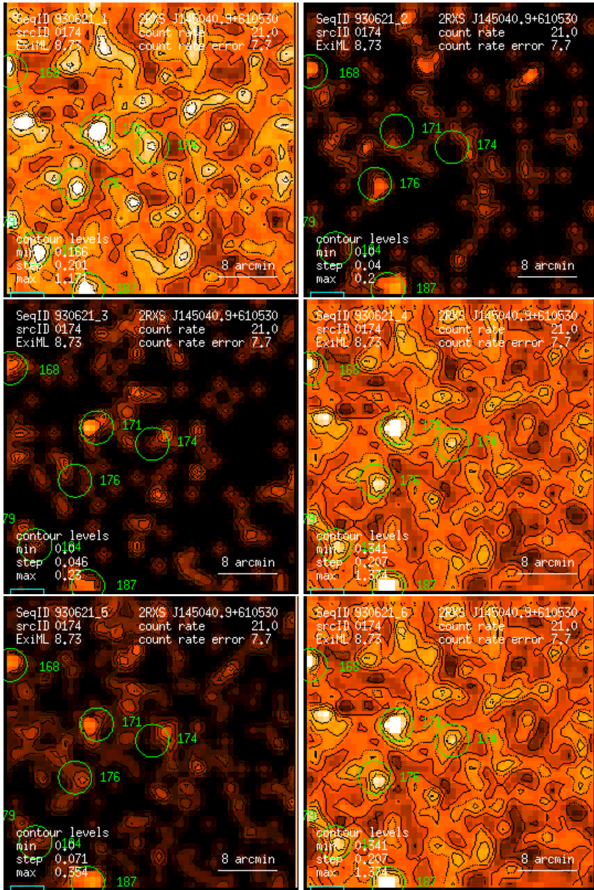
Figure 174: RASS 930621: detection 0174: band rate images, Gaussian filter: (1) PSPC channels 11 – 41, (2) 52 – 90, (3) 91 – 201, (4) 11 – 235, (5) 52 – 201, (6) 11 – 201. Broad band rates in counts/ks. Band rate contour levels in counts/ks/arcmin 2 .
