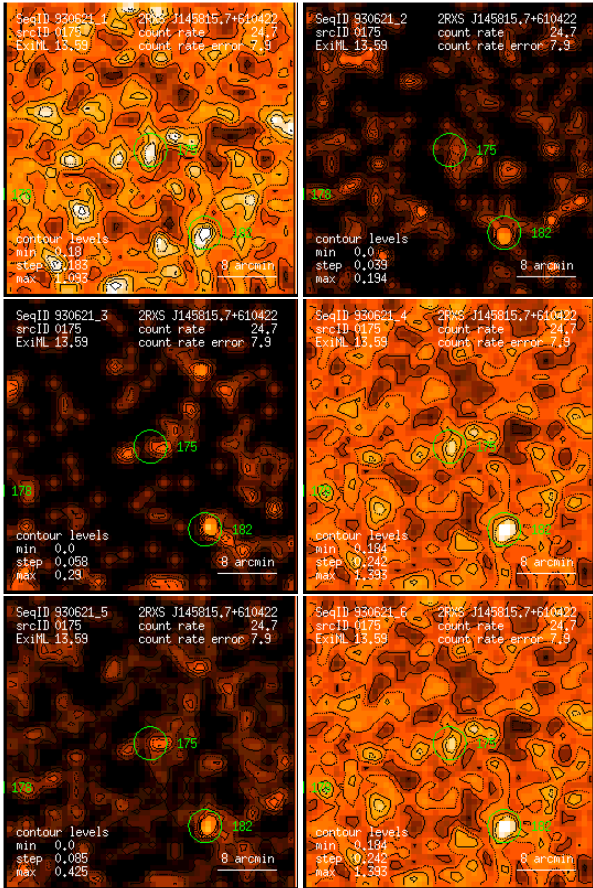
Figure 175: RASS 930621: detection 0175: band rate images, Gaussian filter: (1) PSPC channels 11 – 41, (2) 52 – 90, (3) 91 – 201, (4) 11 – 235, (5) 52 – 201, (6) 11 – 201. Broad band rates in counts/ks. Band rate contour levels in counts/ks/arcmin 2 .
