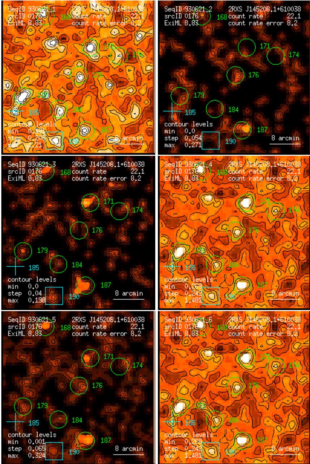
Figure 176: RASS 930621: detection 0176: band rate images, Gaussian filter: (1) PSPC channels 11 – 41, (2) 52 – 90, (3) 91 – 201, (4) 11 – 235, (5) 52 – 201, (6) 11 – 201. Broad band rates in counts/ks. Band rate contour levels in counts/ks/arcmin 2 .
