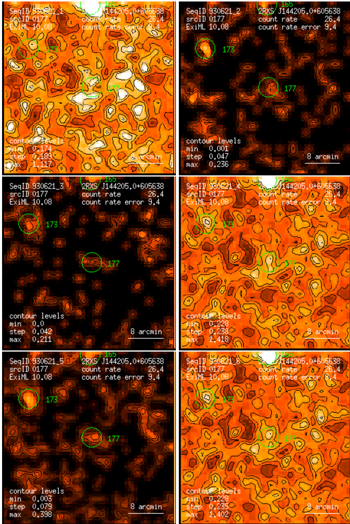
Figure 177: RASS 930621: detection 0177: band rate images, Gaussian filter: (1) PSPC channels 11 – 41, (2) 52 – 90, (3) 91 – 201, (4) 11 – 235, (5) 52 – 201, (6) 11 – 201. Broad band rates in counts/ks. Band rate contour levels in counts/ks/arcmin 2 .
