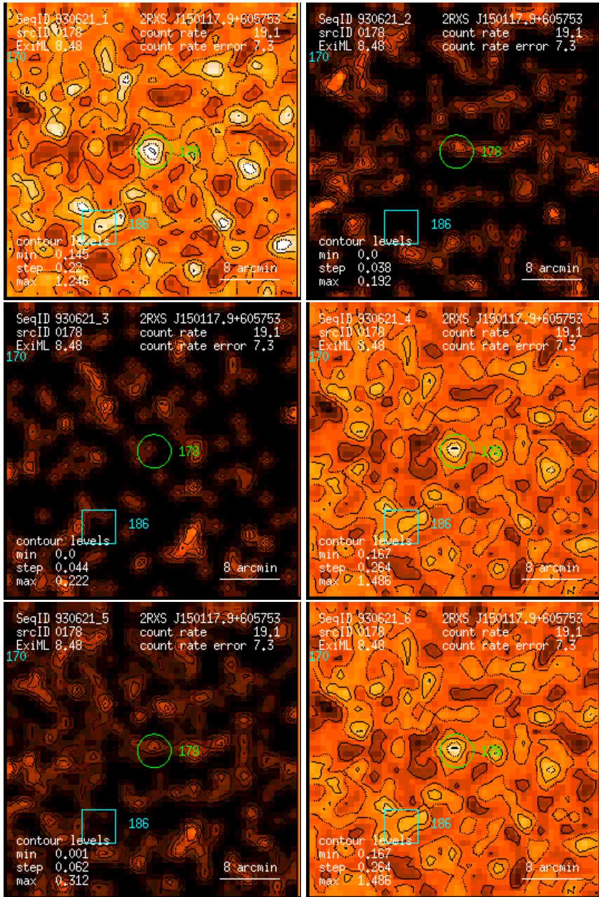
Figure 178: RASS 930621: detection 0178: band rate images, Gaussian filter: (1) PSPC channels 11 – 41, (2) 52 – 90, (3) 91 – 201, (4) 11 – 235, (5) 52 – 201, (6) 11 – 201. Broad band rates in counts/ks. Band rate contour levels in counts/ks/arcmin 2 .
