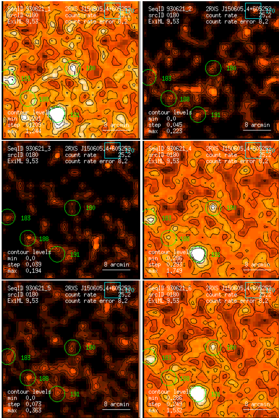
Figure 180: RASS 930621: detection 0180: band rate images, Gaussian filter: (1) PSPC channels 11 – 41, (2) 52 – 90, (3) 91 – 201, (4) 11 – 235, (5) 52 – 201, (6) 11 – 201. Broad band rates in counts/ks. Band rate contour levels in counts/ks/arcmin 2 .
