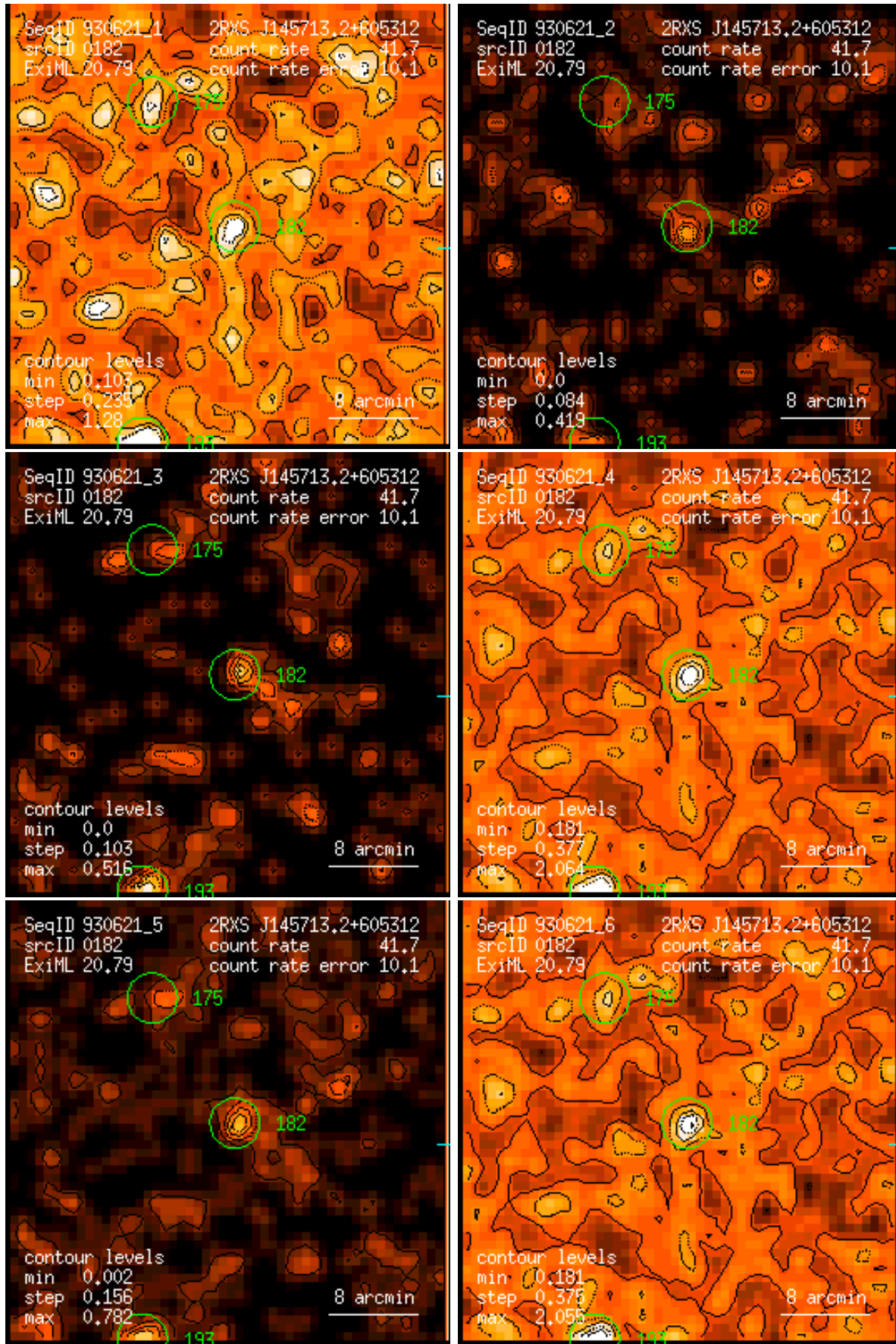
Figure 182: RASS 930621: detection 0182: band rate images, Gaussian filter: (1) PSPC channels 11 – 41, (2) 52 – 90, (3) 91 – 201, (4) 11 – 235, (5) 52 – 201, (6) 11 – 201. Broad band rates in counts/ks. Band rate contour levels in counts/ks/arcmin 2 .
