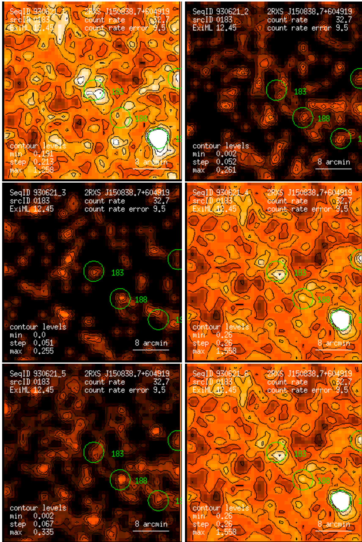
Figure 183: RASS 930621: detection 0183: band rate images, Gaussian filter: (1) PSPC channels 11 – 41, (2) 52 – 90, (3) 91 – 201, (4) 11 – 235, (5) 52 – 201, (6) 11 – 201. Broad band rates in counts/ks. Band rate contour levels in counts/ks/arcmin 2 .
