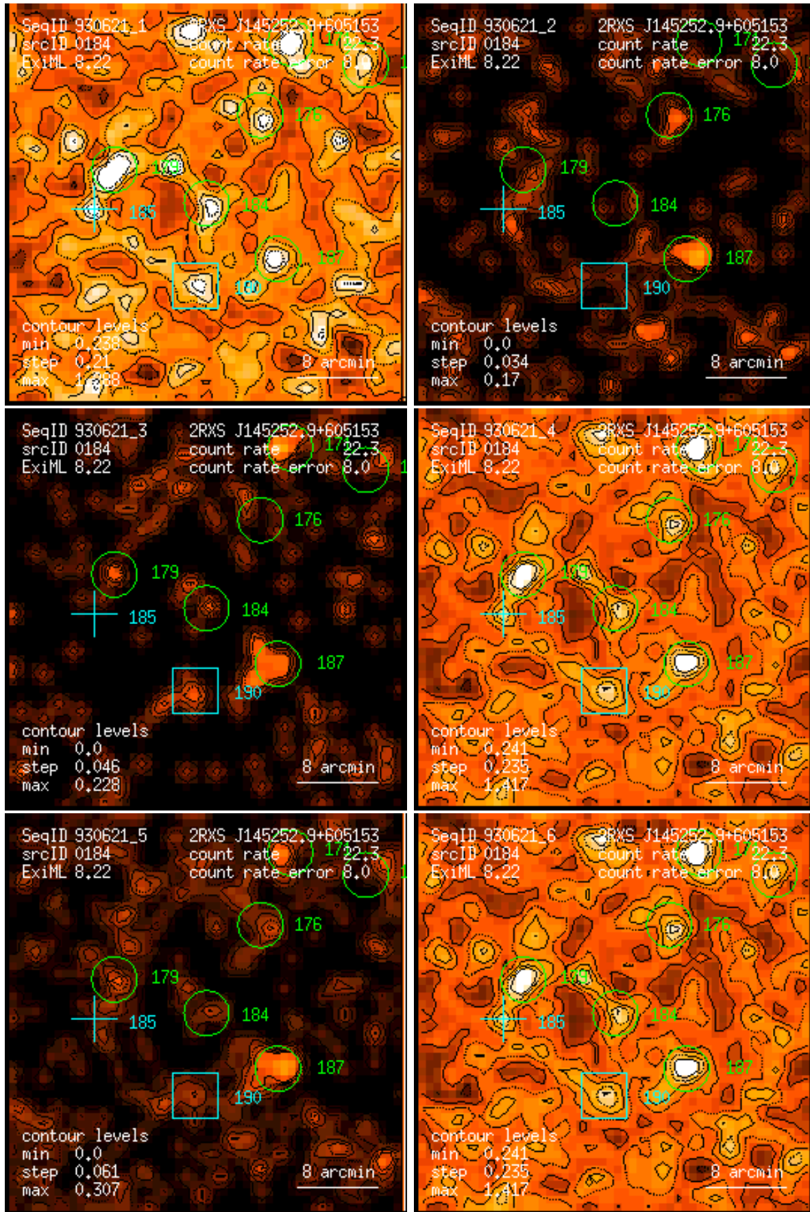
Figure 184: RASS 930621: detection 0184: band rate images, Gaussian filter: (1) PSPC channels 11 – 41, (2) 52 – 90, (3) 91 – 201, (4) 11 – 235, (5) 52 – 201, (6) 11 – 201. Broad band rates in counts/ks. Band rate contour levels in counts/ks/arcmin 2 .
