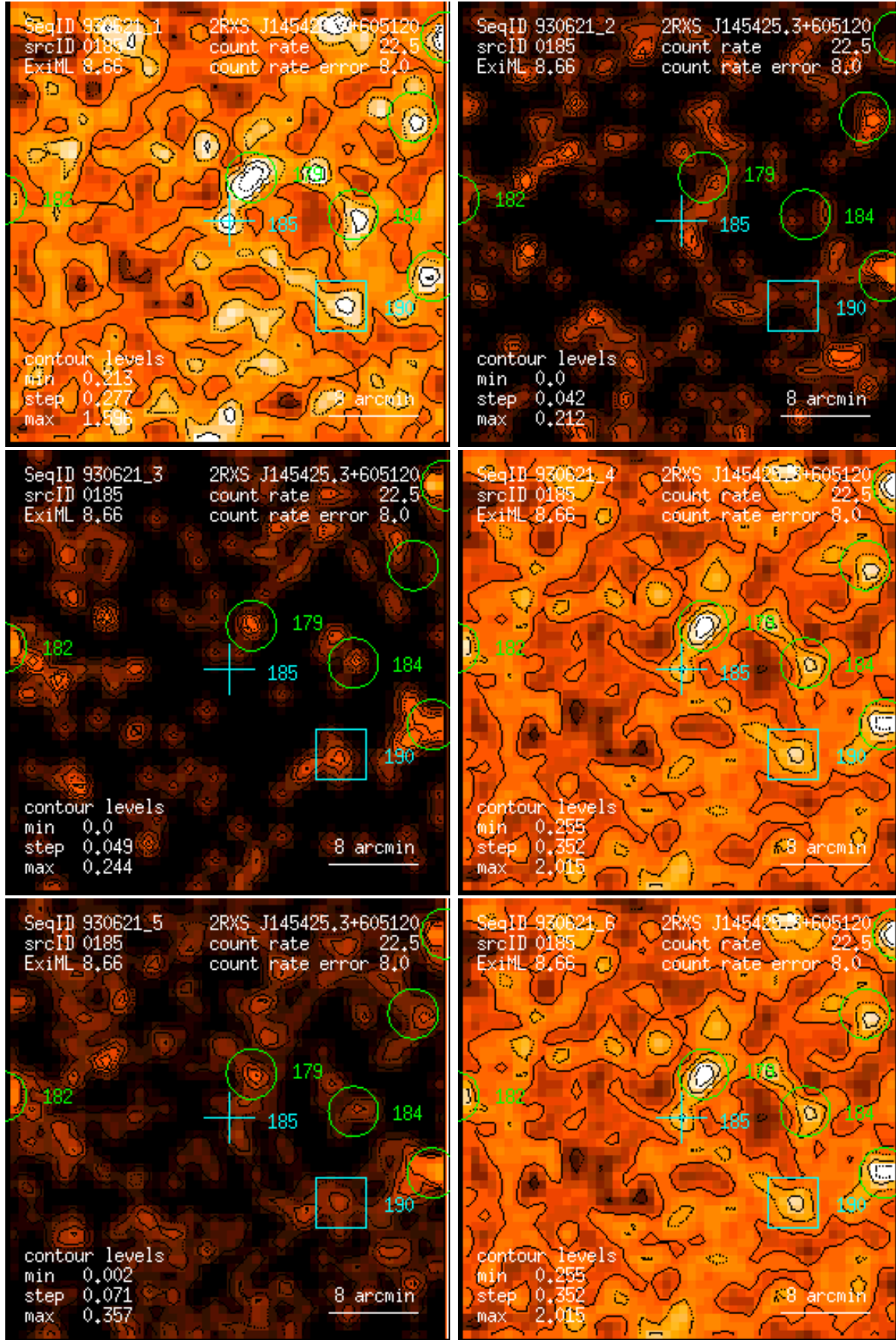
Figure 185: RASS 930621: detection 0185: band rate images, Gaussian filter: (1) PSPC channels 11 – 41, (2) 52 – 90, (3) 91 – 201, (4) 11 – 235, (5) 52 – 201, (6) 11 – 201. Broad band rates in counts/ks. Band rate contour levels in counts/ks/arcmin 2 .
