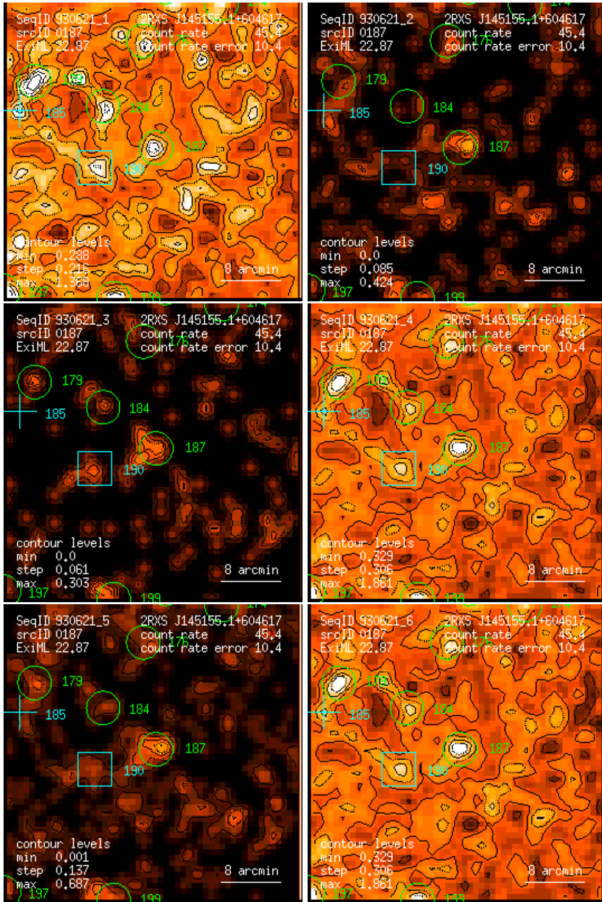
Figure 187: RASS 930621: detection 0187: band rate images, Gaussian filter: (1) PSPC channels 11 – 41, (2) 52 – 90, (3) 91 – 201, (4) 11 – 235, (5) 52 – 201, (6) 11 – 201. Broad band rates in counts/ks. Band rate contour levels in counts/ks/arcmin 2 .
