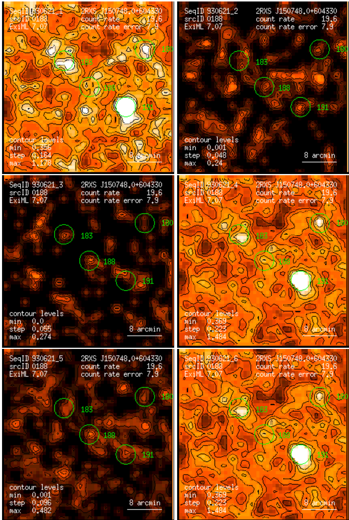
Figure 188: RASS 930621: detection 0188: band rate images, Gaussian filter: (1) PSPC channels 11 – 41, (2) 52 – 90, (3) 91 – 201, (4) 11 – 235, (5) 52 – 201, (6) 11 – 201. Broad band rates in counts/ks. Band rate contour levels in counts/ks/arcmin 2 .
