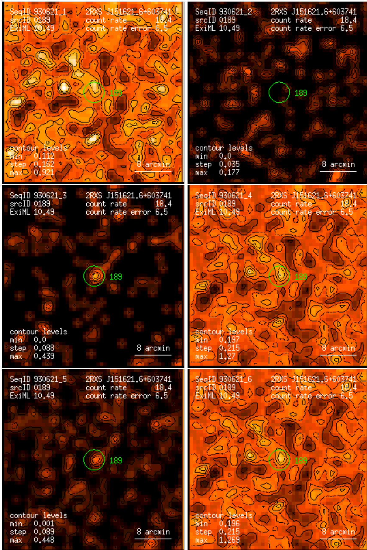
Figure 189: RASS 930621: detection 0189: band rate images, Gaussian filter: (1) PSPC channels 11 – 41, (2) 52 – 90, (3) 91 – 201, (4) 11 – 235, (5) 52 – 201, (6) 11 – 201. Broad band rates in counts/ks. Band rate contour levels in counts/ks/arcmin 2 .
