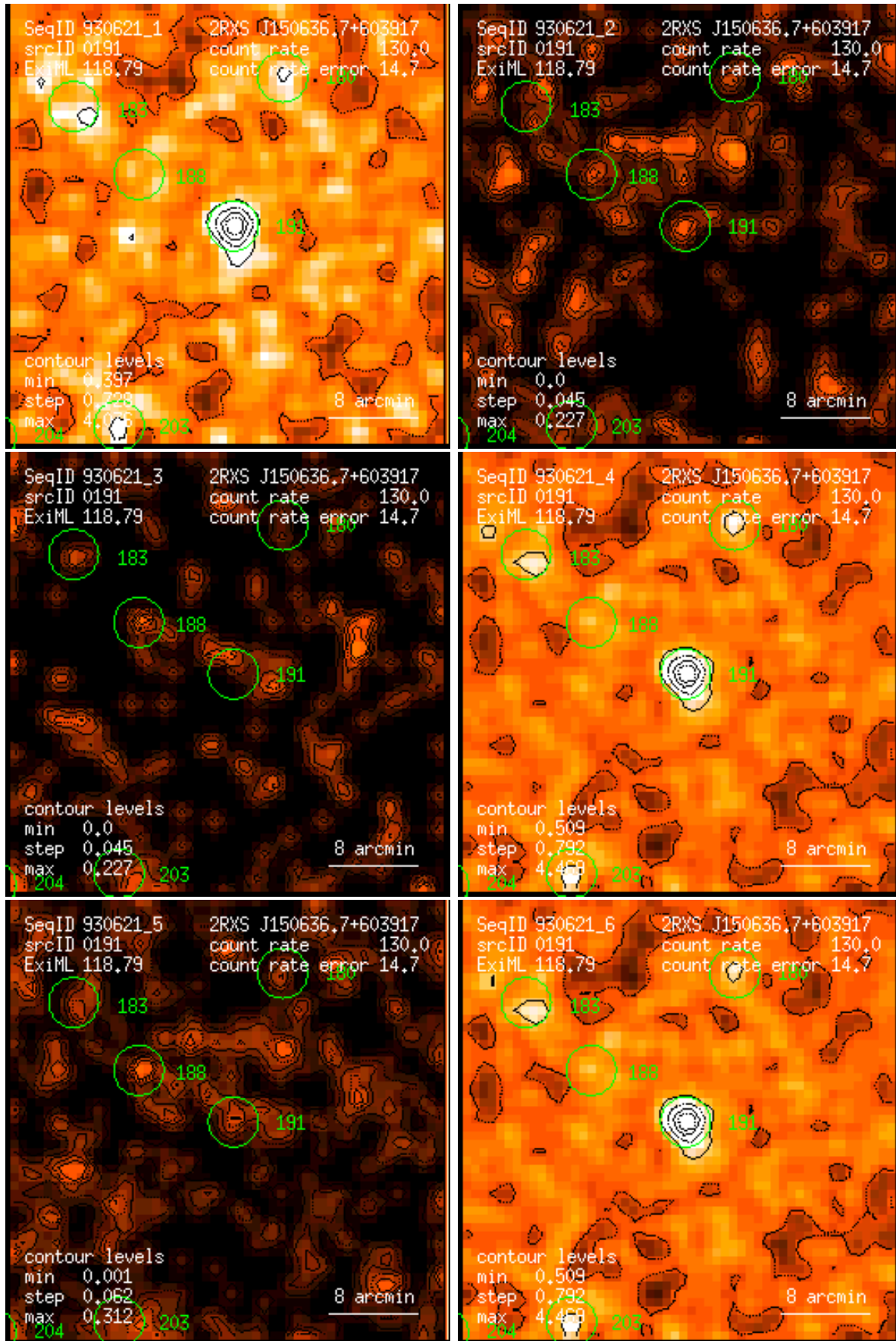
Figure 191: RASS 930621: detection 0191: band rate images, Gaussian filter: (1) PSPC channels 11 – 41, (2) 52 – 90, (3) 91 – 201, (4) 11 – 235, (5) 52 – 201, (6) 11 – 201. Broad band rates in counts/ks. Band rate contour levels in counts/ks/arcmin 2 .
