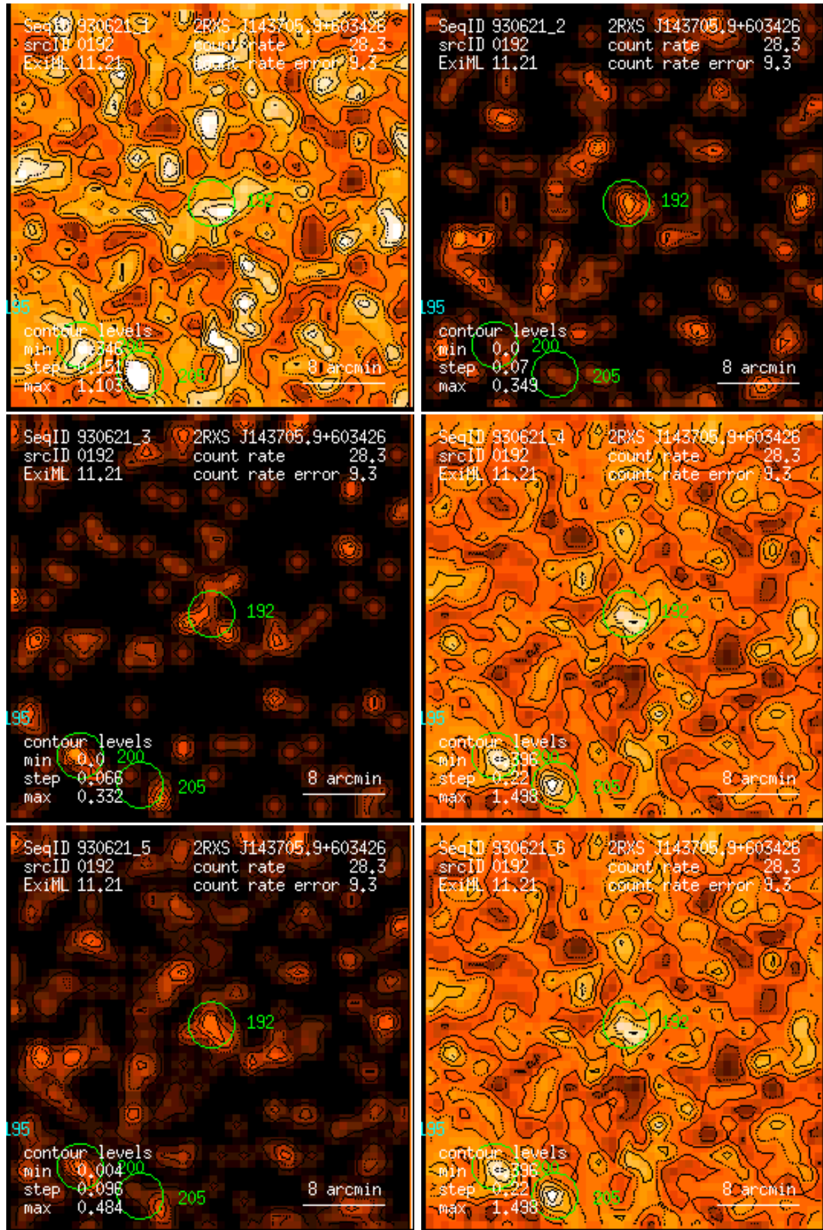
Figure 192: RASS 930621: detection 0192: band rate images, Gaussian filter: (1) PSPC channels 11 – 41, (2) 52 – 90, (3) 91 – 201, (4) 11 – 235, (5) 52 – 201, (6) 11 – 201. Broad band rates in counts/ks. Band rate contour levels in counts/ks/arcmin 2 .
