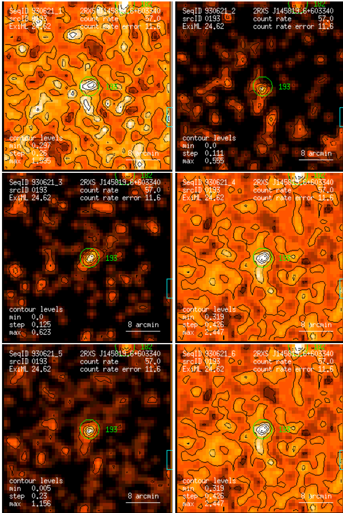
Figure 193: RASS 930621: detection 0193: band rate images, Gaussian filter: (1) PSPC channels 11 – 41, (2) 52 – 90, (3) 91 – 201, (4) 11 – 235, (5) 52 – 201, (6) 11 – 201. Broad band rates in counts/ks. Band rate contour levels in counts/ks/arcmin 2 .
