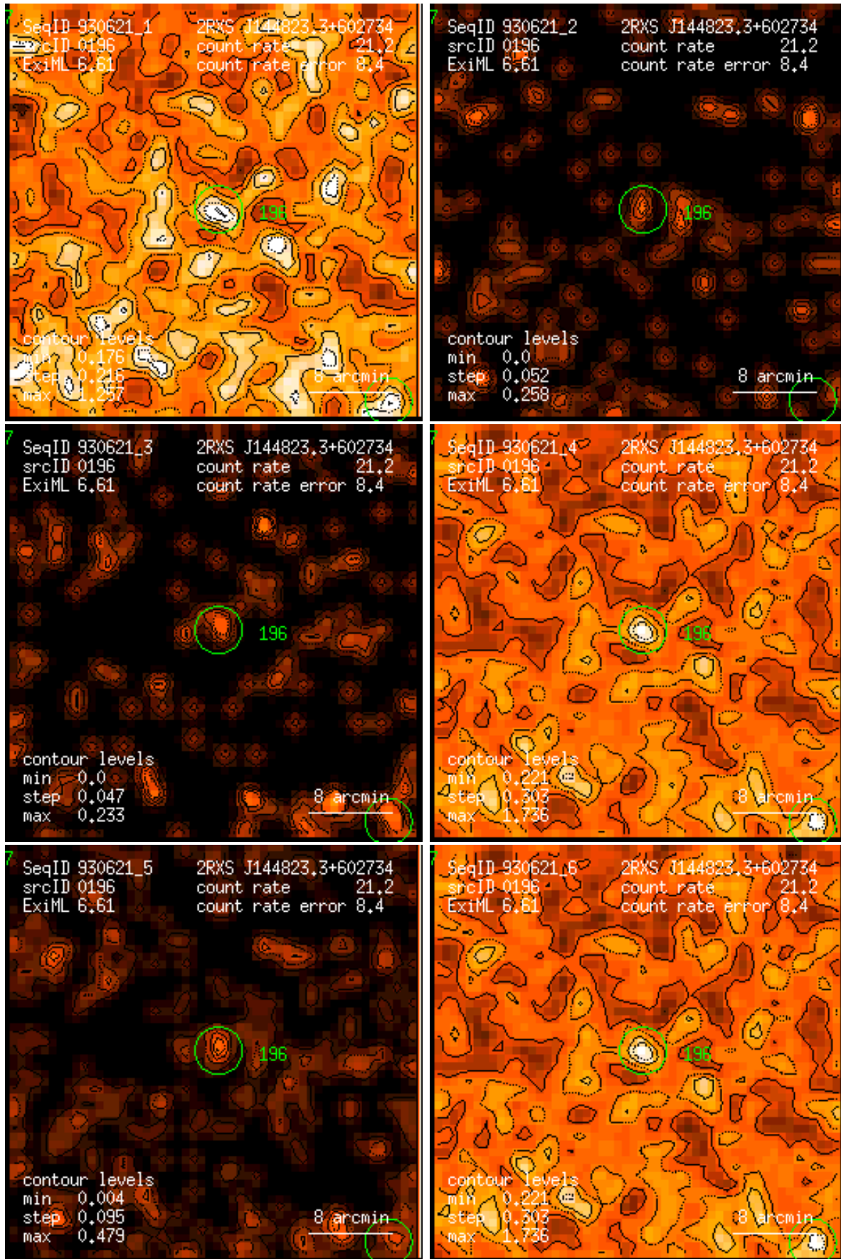
Figure 196: RASS 930621: detection 0196: band rate images, Gaussian filter: (1) PSPC channels 11 – 41, (2) 52 – 90, (3) 91 – 201, (4) 11 – 235, (5) 52 – 201, (6) 11 – 201. Broad band rates in counts/ks. Band rate contour levels in counts/ks/arcmin 2 .
