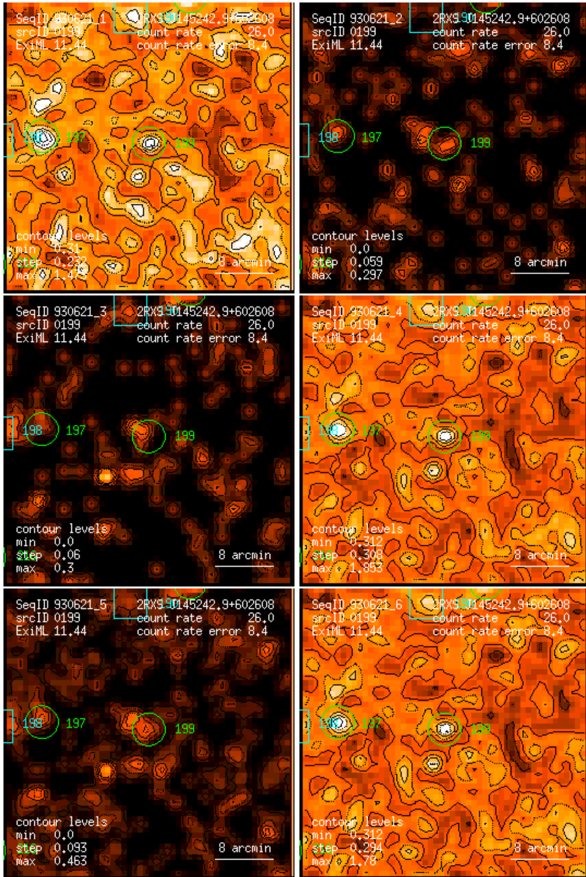
Figure 199: RASS 930621: detection 0199: band rate images, Gaussian filter: (1) PSPC channels 11 – 41, (2) 52 – 90, (3) 91 – 201, (4) 11 – 235, (5) 52 – 201, (6) 11 – 201. Broad band rates in counts/ks. Band rate contour levels in counts/ks/arcmin 2 .
